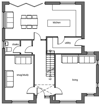
ground floor plan (orangery removed)
