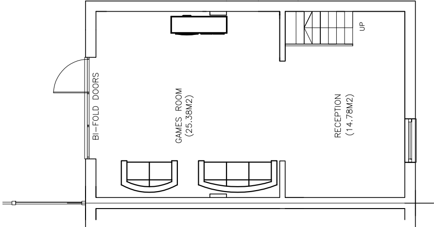
FLOOR AREA 40.16M2 (USEABLE SPACE –EXC STAIR) EXISTING LOWER GROUND FLOOR PLAN
