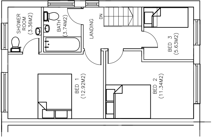
PROPOSED FIRST FLOOR PLAN (NO MATERIAL CHANGE)
