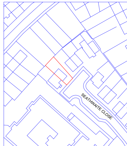
Location Plan 1 : 1250
