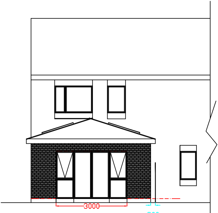
Rear Elevation
