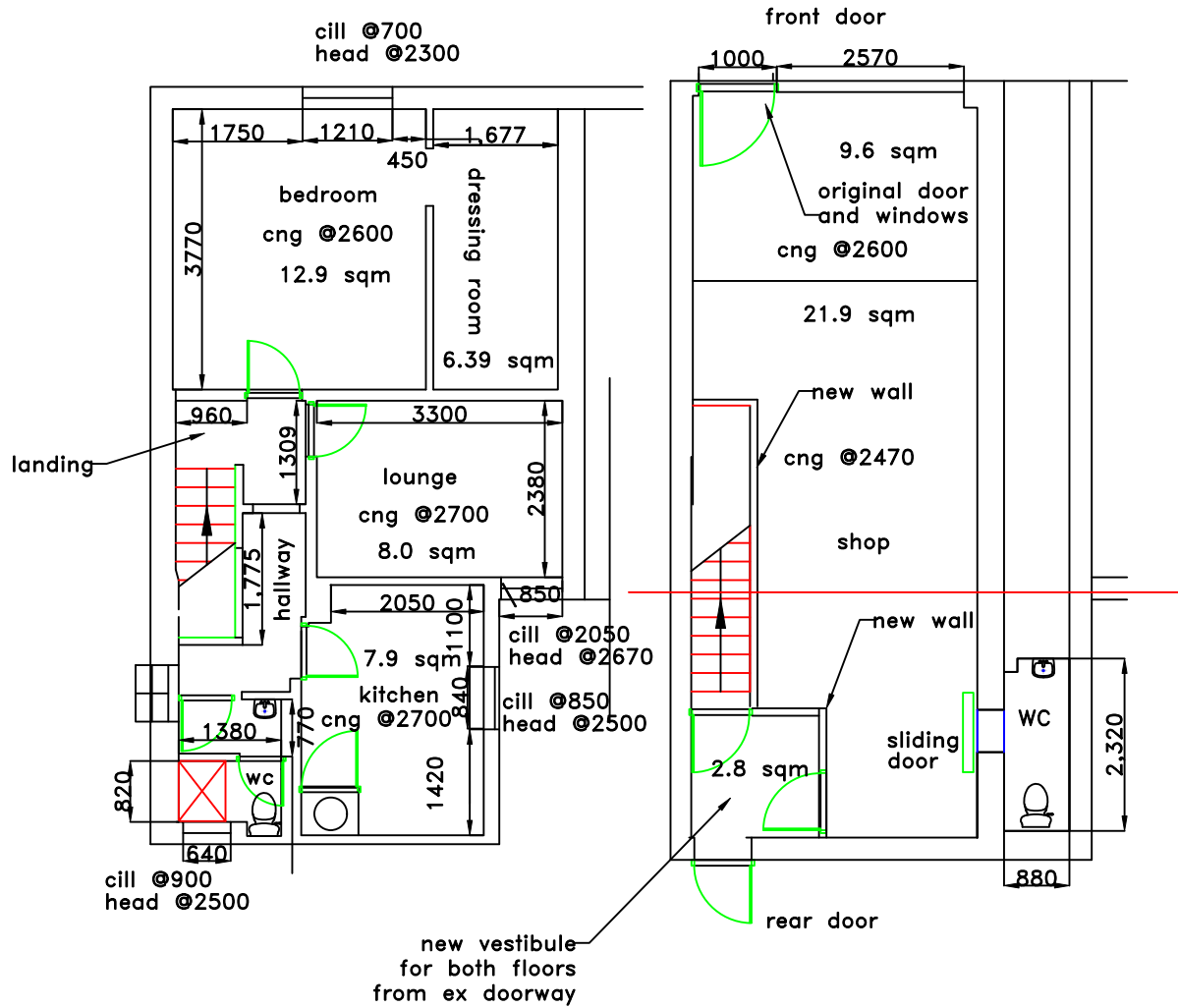
PROPOSED FIRST FLOOR
