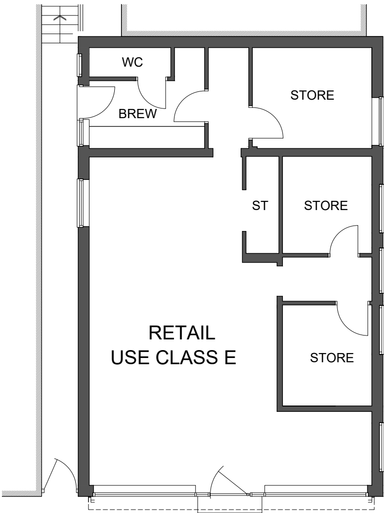
Floor plan as Existing
