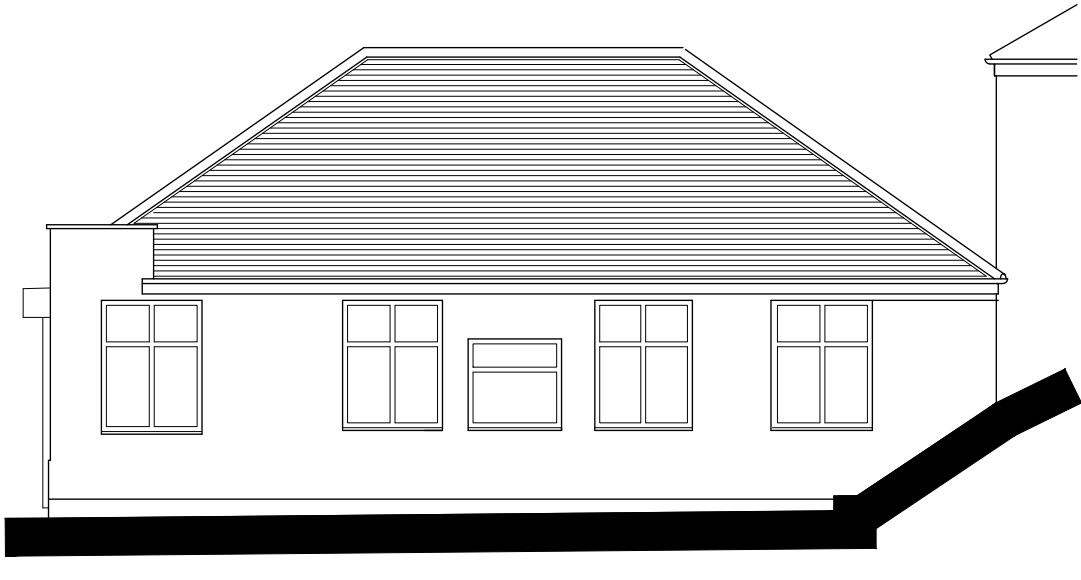
Side Elevation to 217 Manchester New Road as Existing
