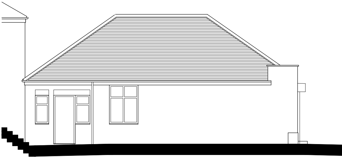
Side Elevation to 213 Manchester New Road as Existing
