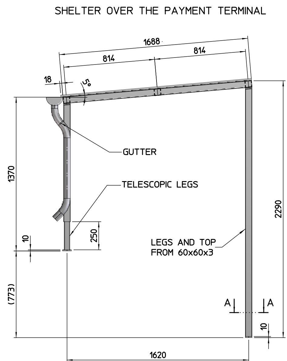
VISTA ANTERIORE - front view1 SCALE 1:20
