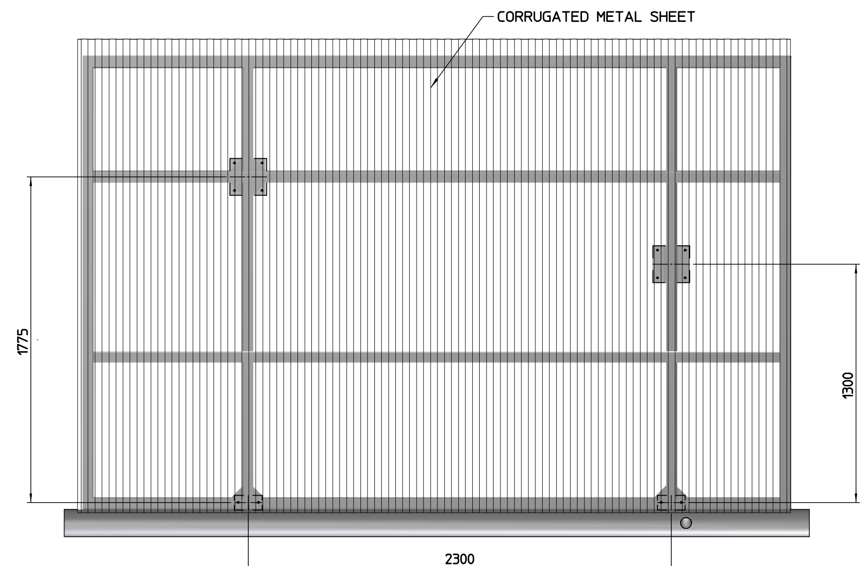
VIEW C SCALE 1:20
