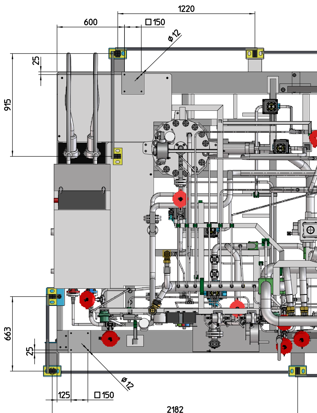
DETAIL-D2 SCALE 1:20
