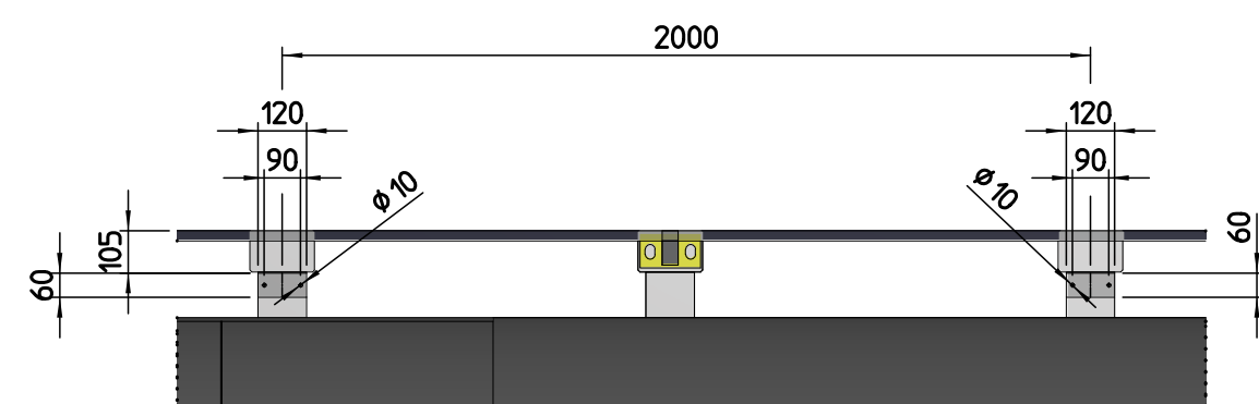
DETAIL-D1 SCALE 1:20
