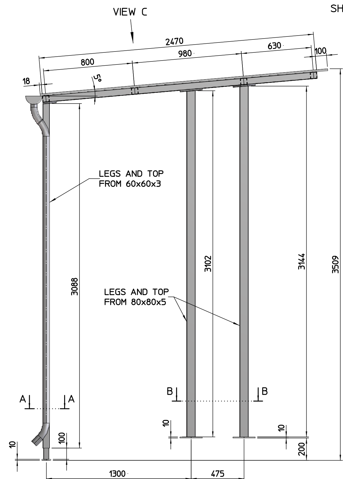
VISTA ANTERIORE - front view3 SCALE 1:20
