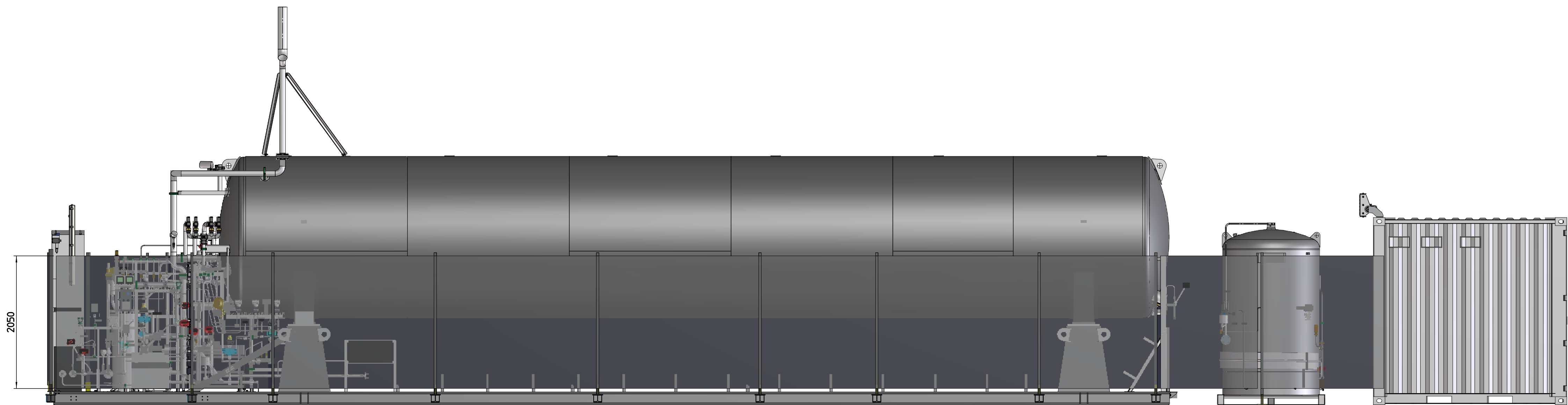
VISTA ANTERIORE - front view2 SCALE 1:40
