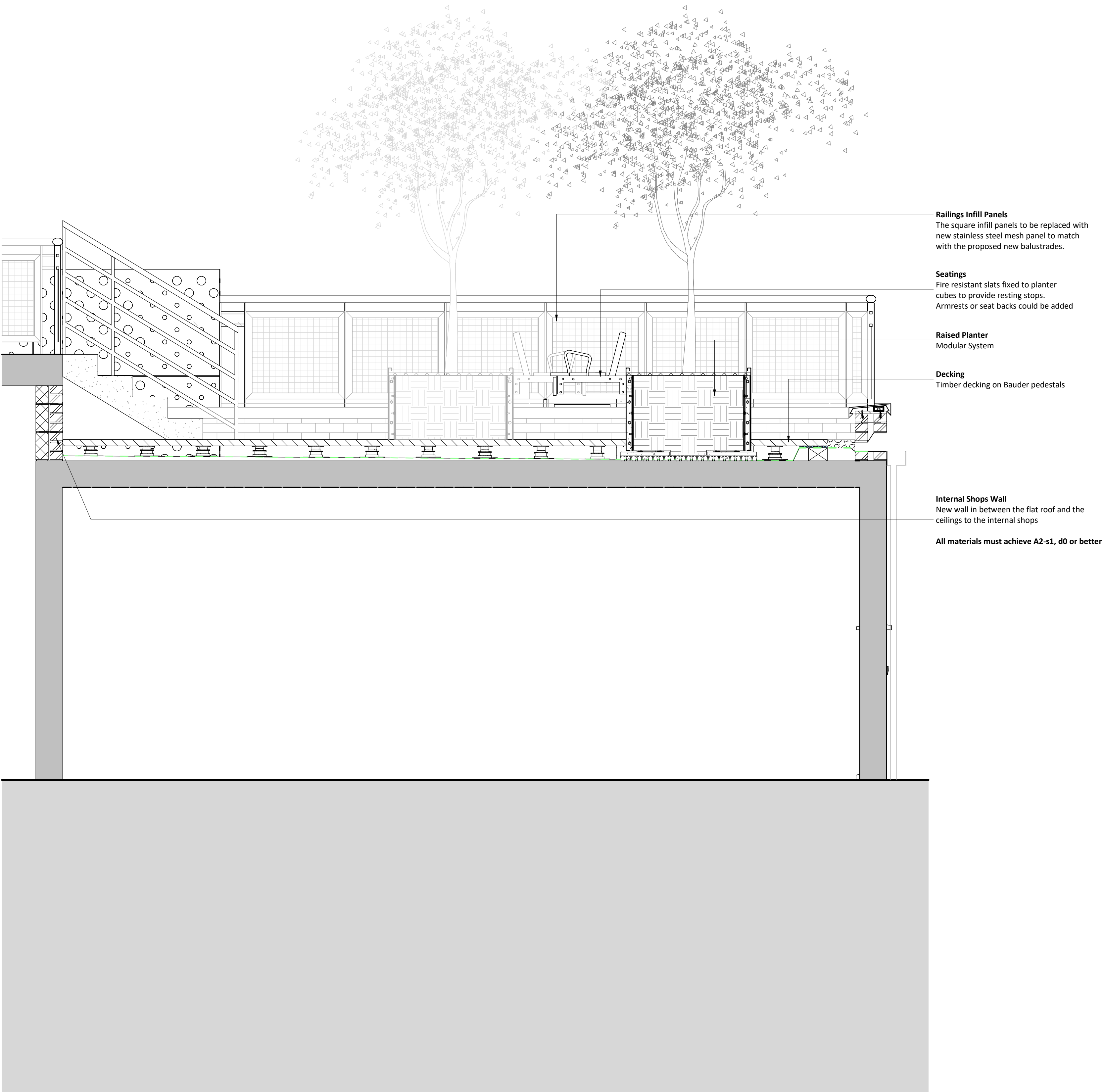
Roof Garden Section 1 : 20
