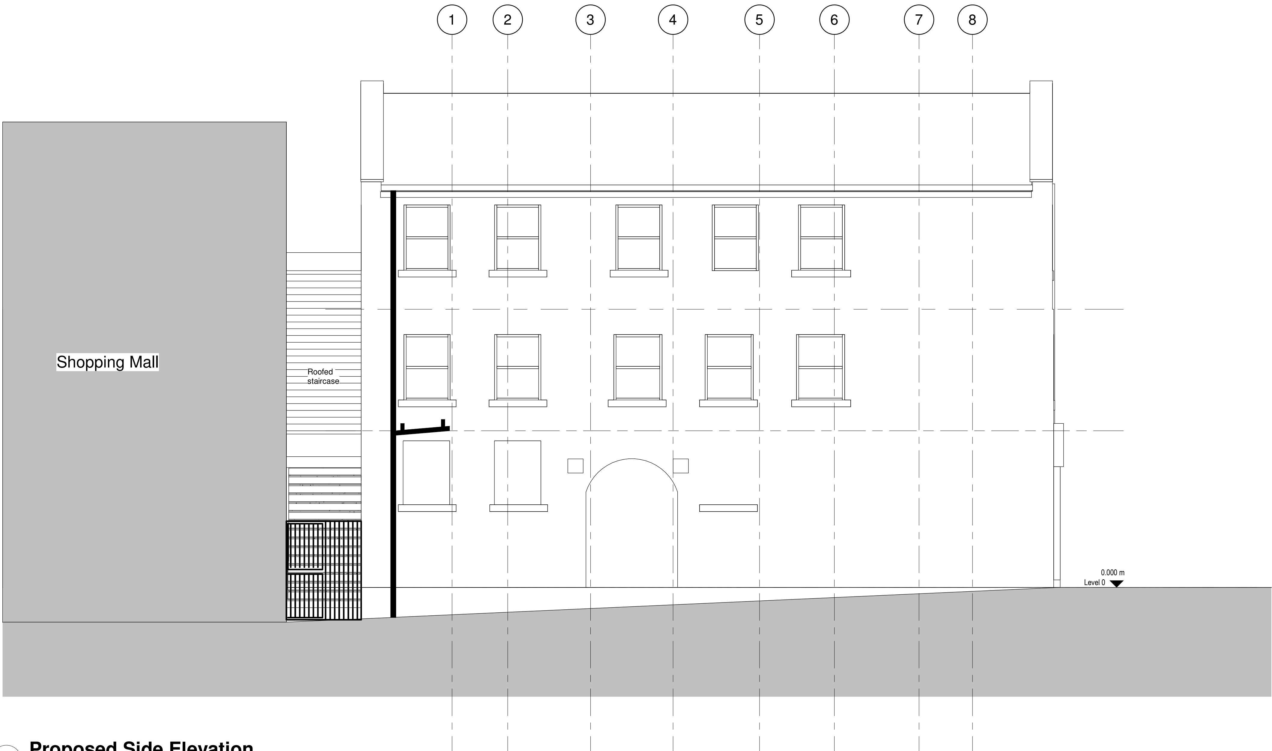
1 Proposed Side Elevation 1 : 50
