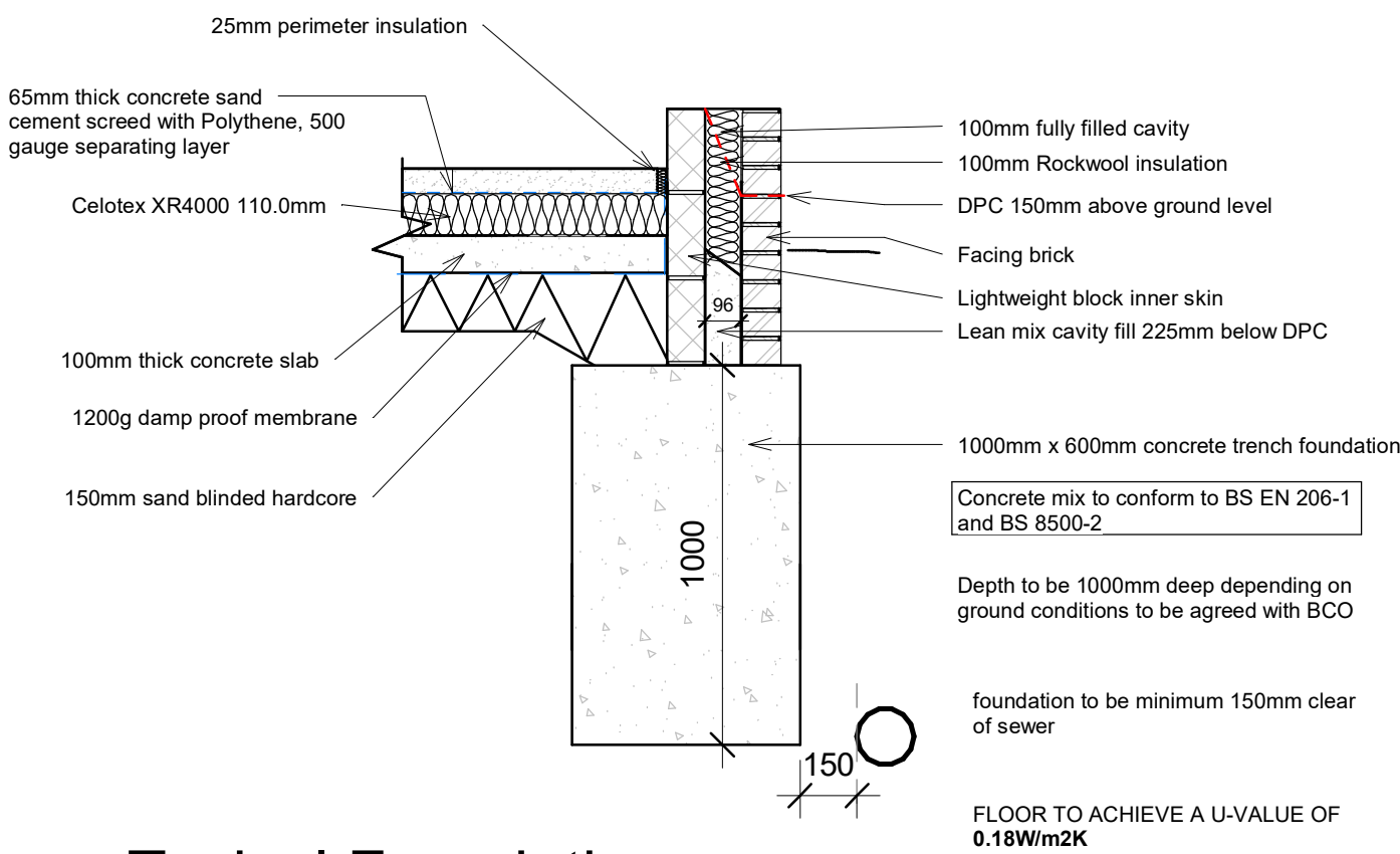
4 Typical Foundation 1 : 20
