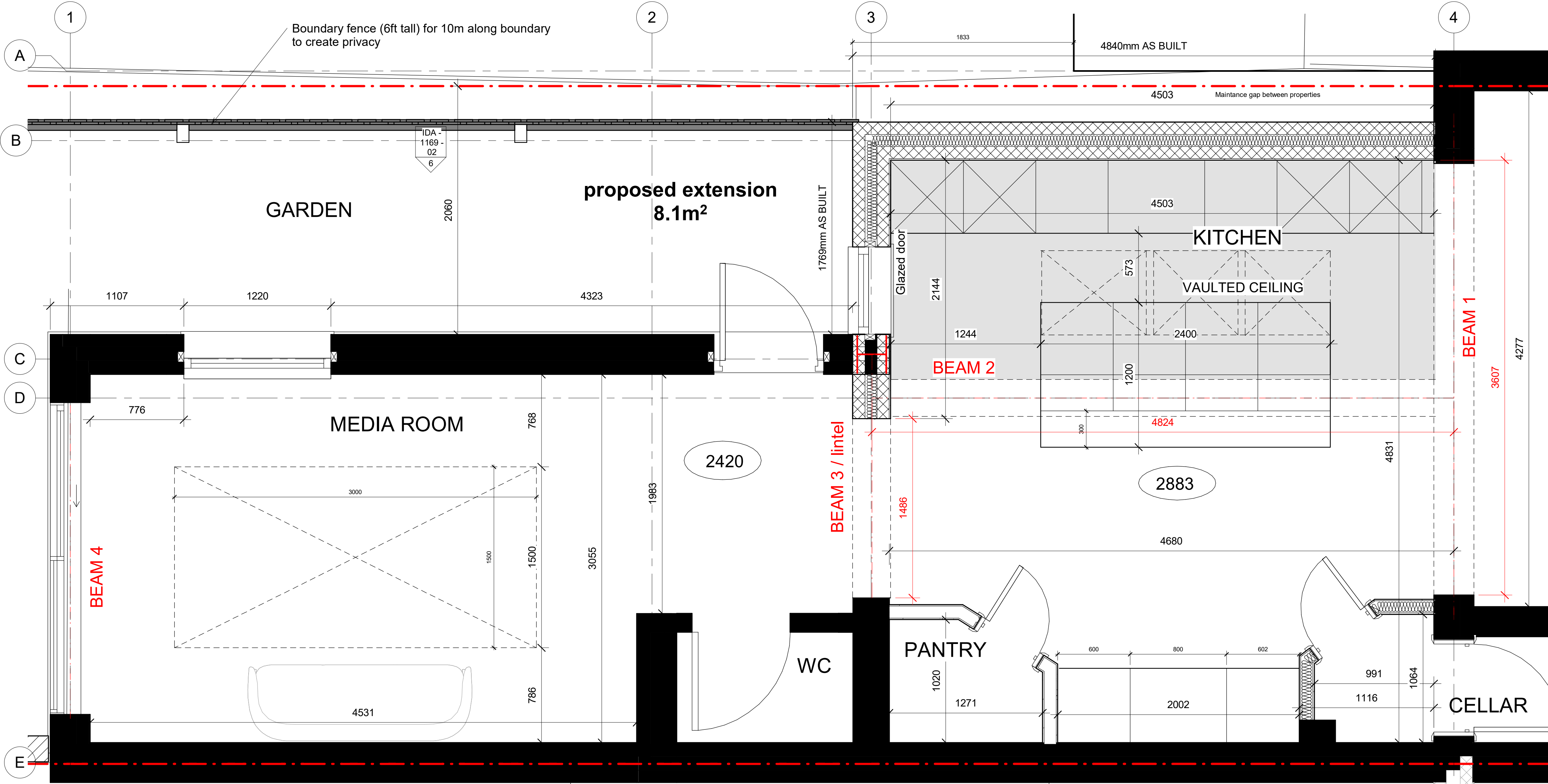
1 Ground Floor Detailed 1 : 20
