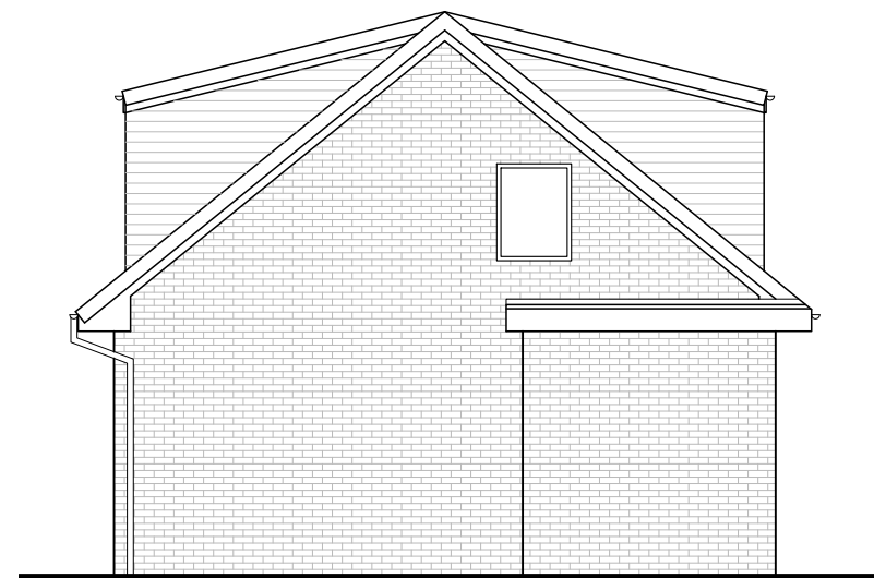
Side Elevation - 1:100
