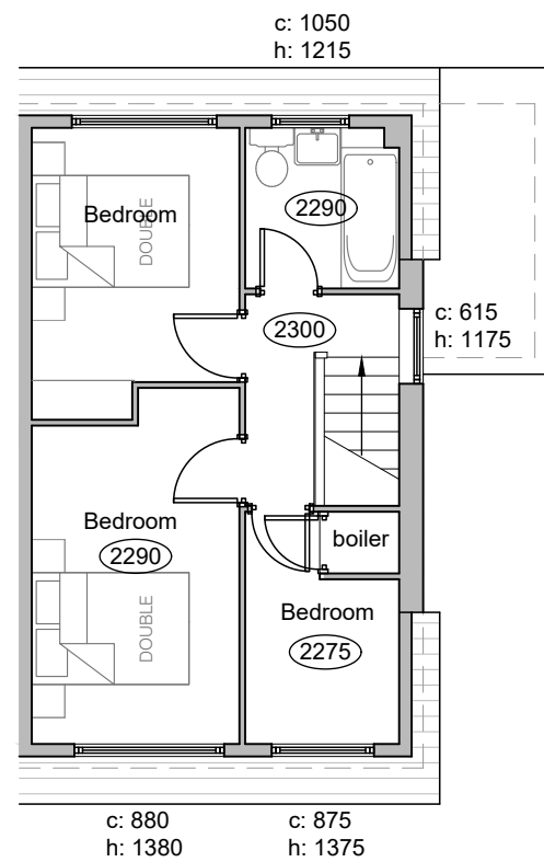
First Floor - 1:100
