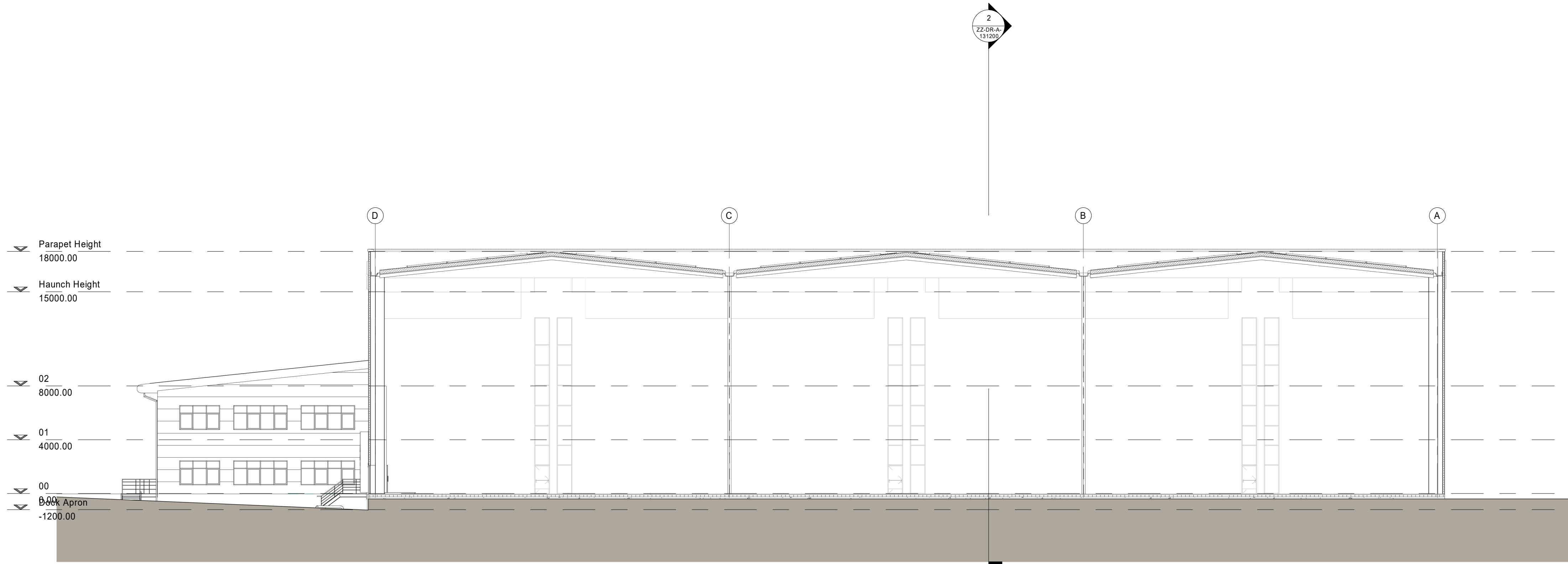
Planning Warehouse Section AA 1 : 200
