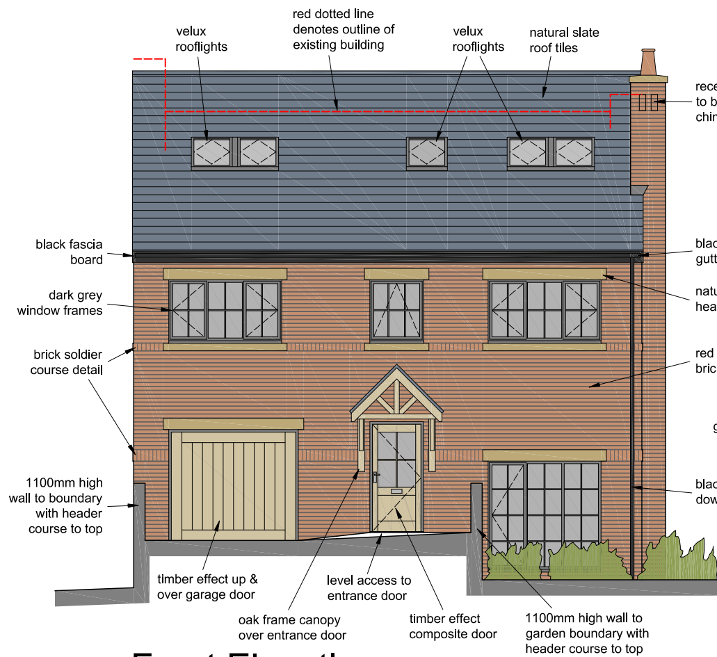
Front Elevation
