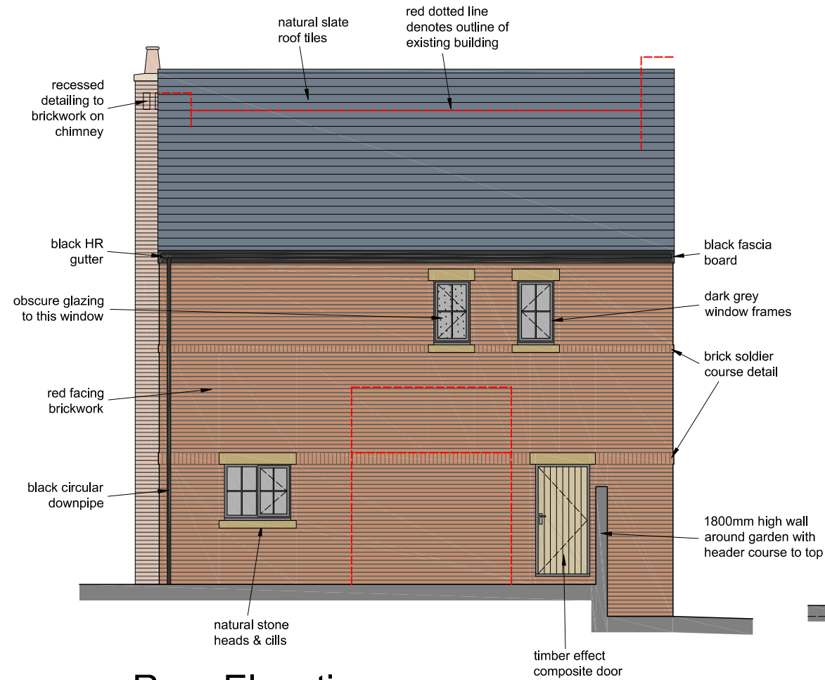
Rear Elevation
