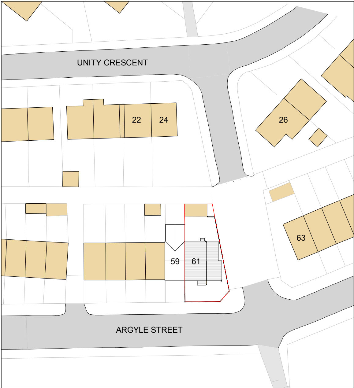
2. Site - Block Plan Proposed 1 : 500
