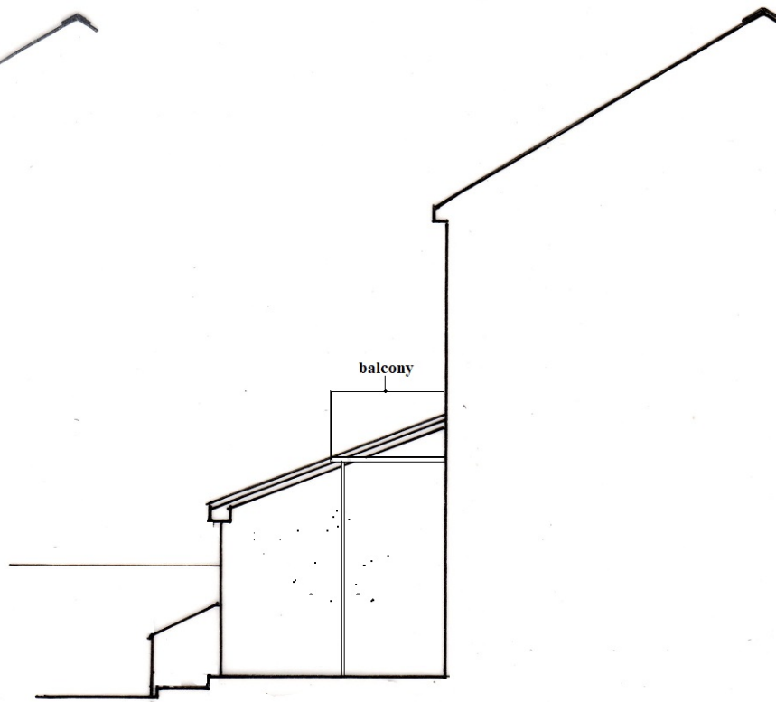
Existing Side Elevation towards 208
