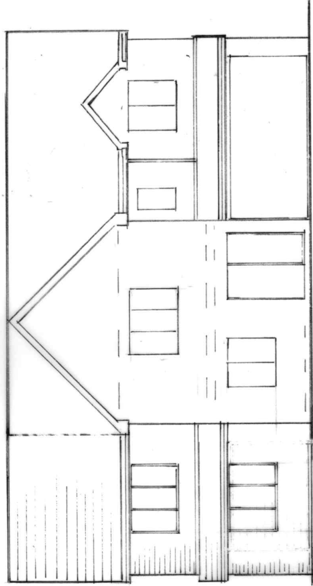
FRONT ELEVATION (PROPOSED)
