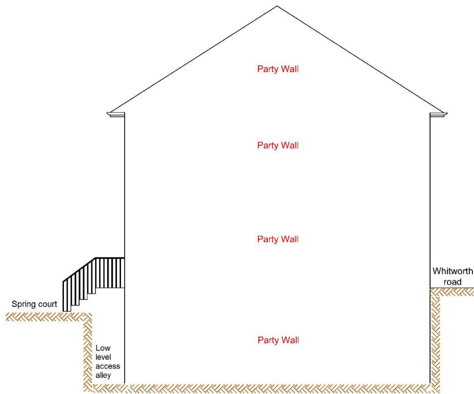
PROPOSED NEIGHBOURING ELEVATION A 1:50 @ A1
