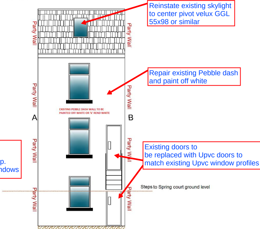
PROPOSED REAR ELEVATION 1:50 @ A1
