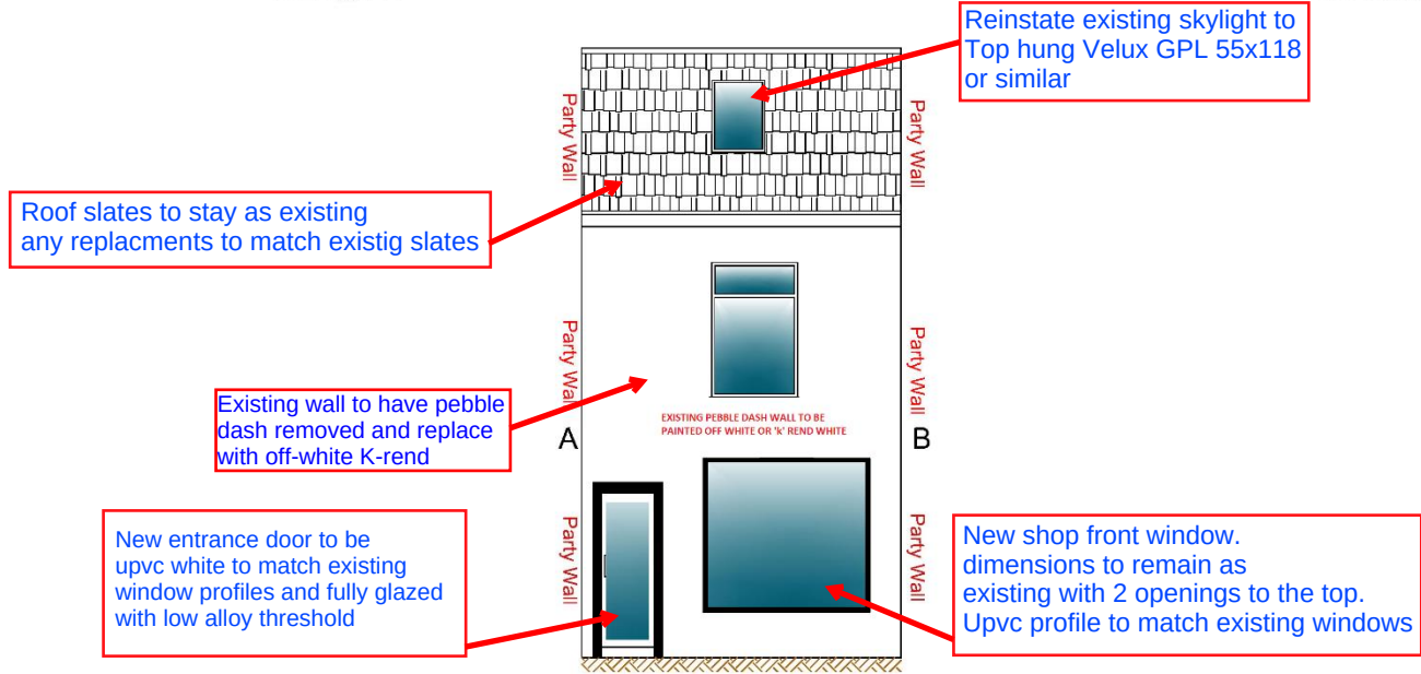
PROPOSED NEIGHBOURING ELEVATION A 1:50 @ A1
