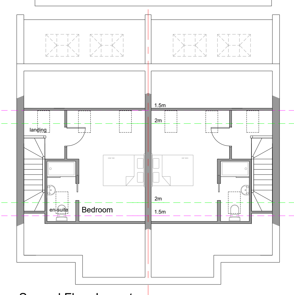
Second Floor Layout
