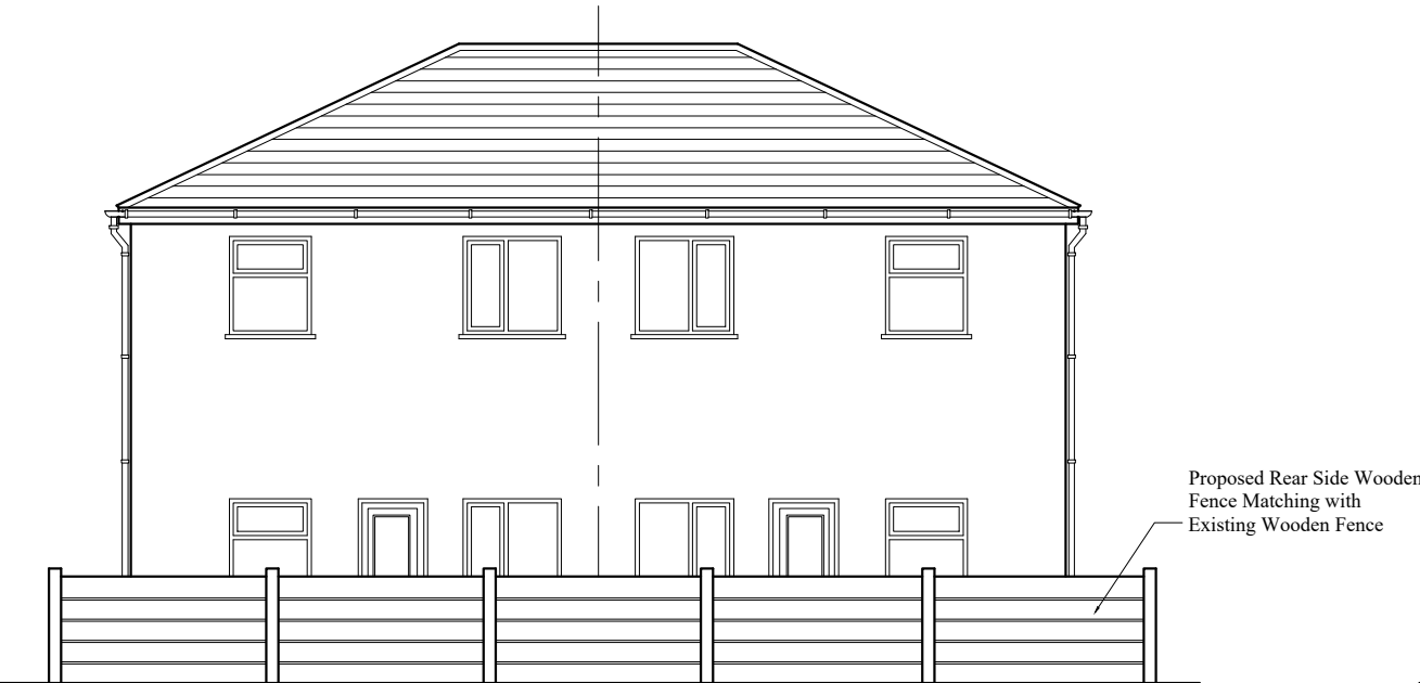
PROPOSED REAR ELEVATION WITH BOUNDARY WALL
