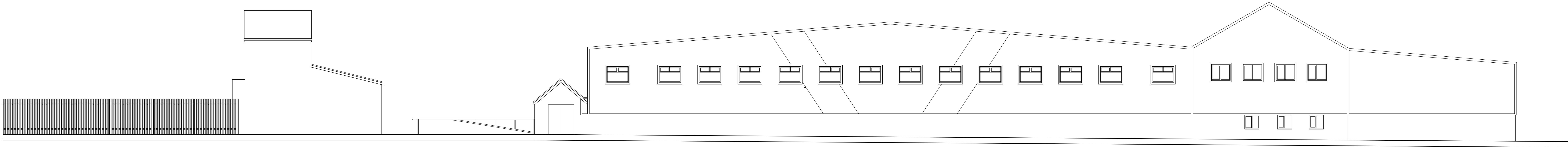
EXISTING STREET SCENE ALONG BUCKLEY ROADscale 1:100
