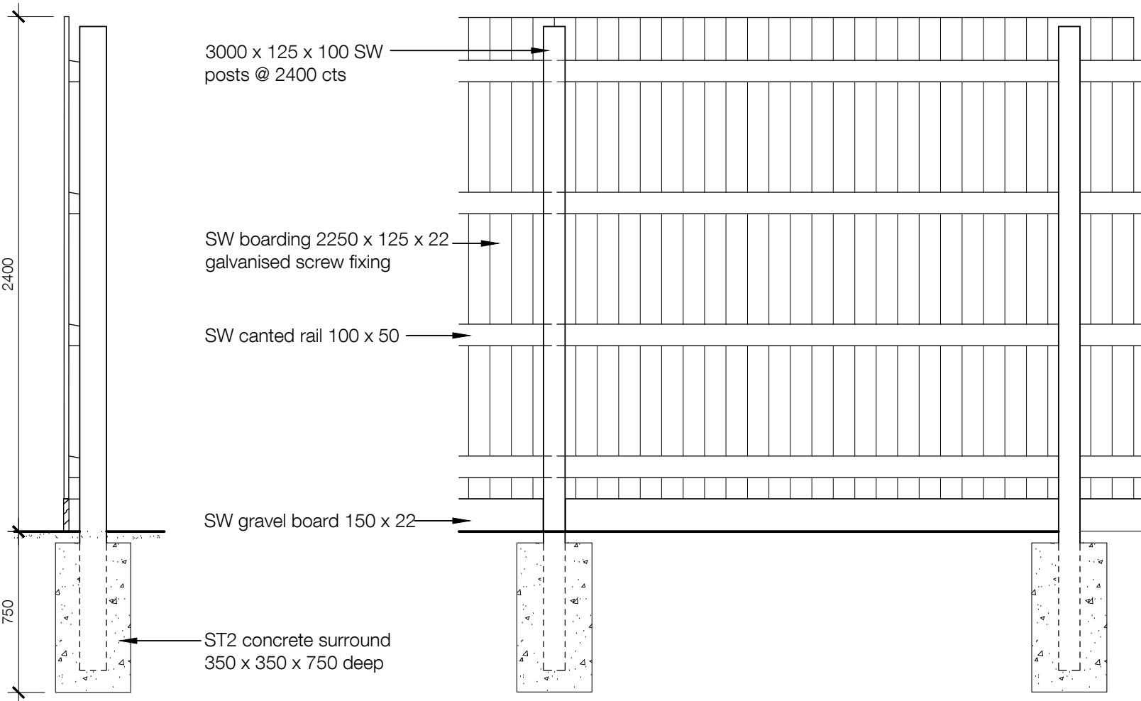
Section Proposed Timber fence to western boundary 1:25
