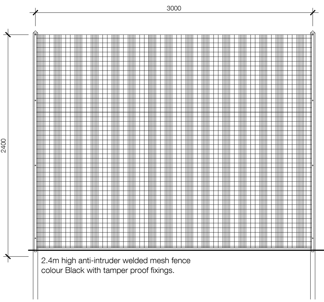
Proposed Weldmesh fence to western boundary 1:25
