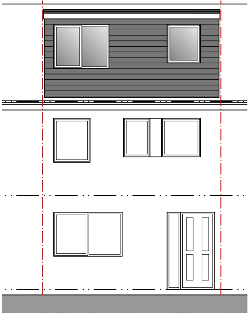
North Facing Rear Elevation
