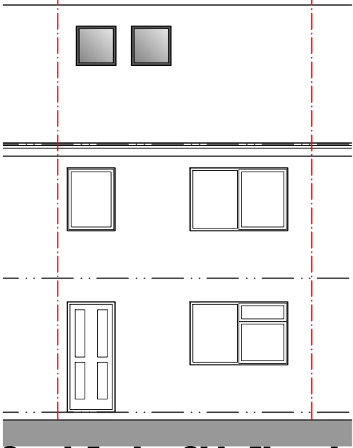
South Facing Side Elevation
