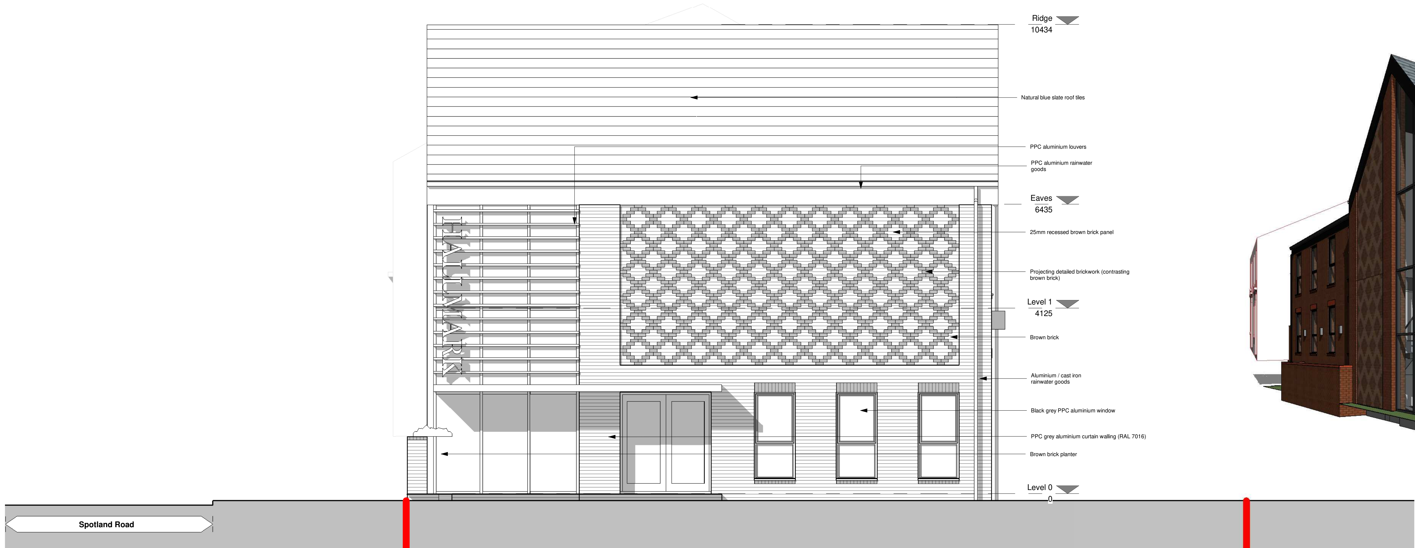
2 Proposed West Elevation
