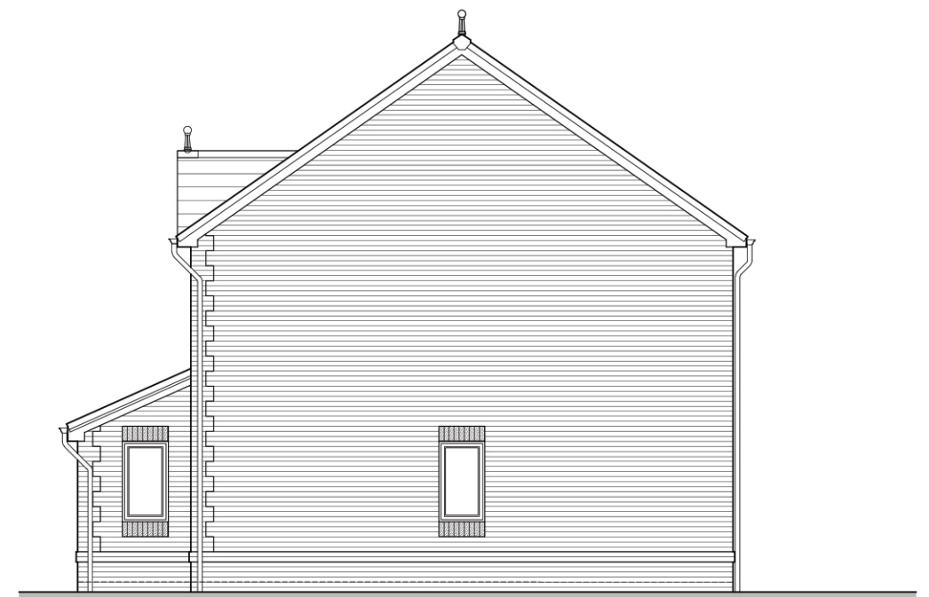
Side Elevation
