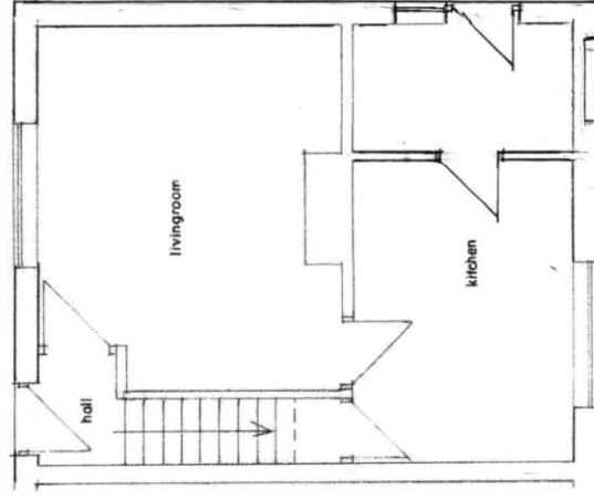
G.F. PLAN (EXISTING)
