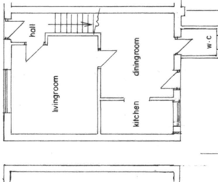
G.F. PLAN (EXISTING)
