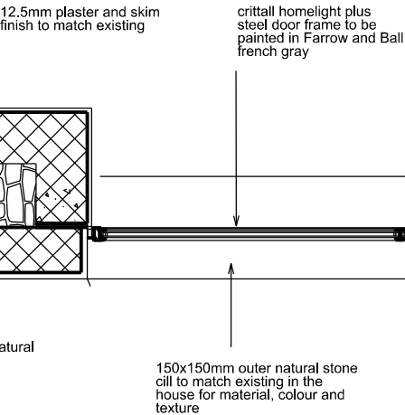
SECTION PLAN
