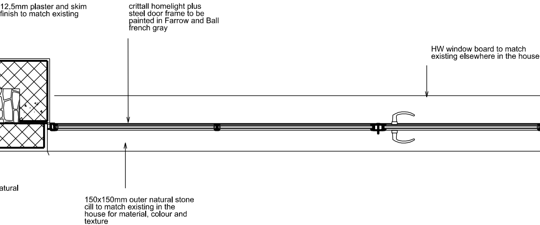
SECTION PLAN
