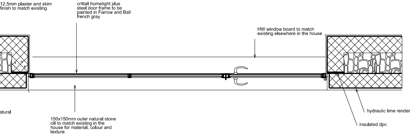
SECTION PLAN
