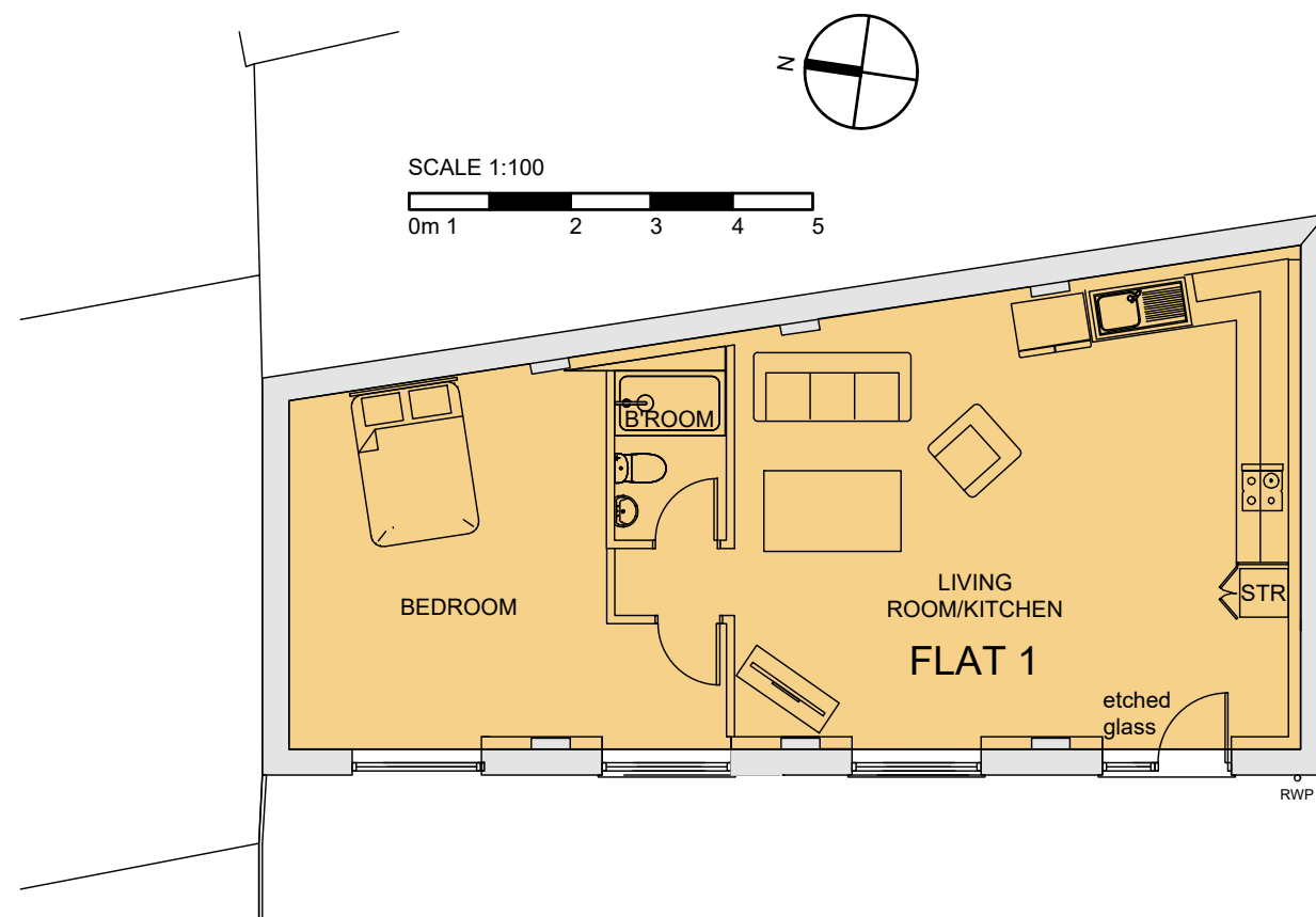
GROUND FLOOR PLAN - (SINGLE STOREY) Proposed GIA: 66 sqm
