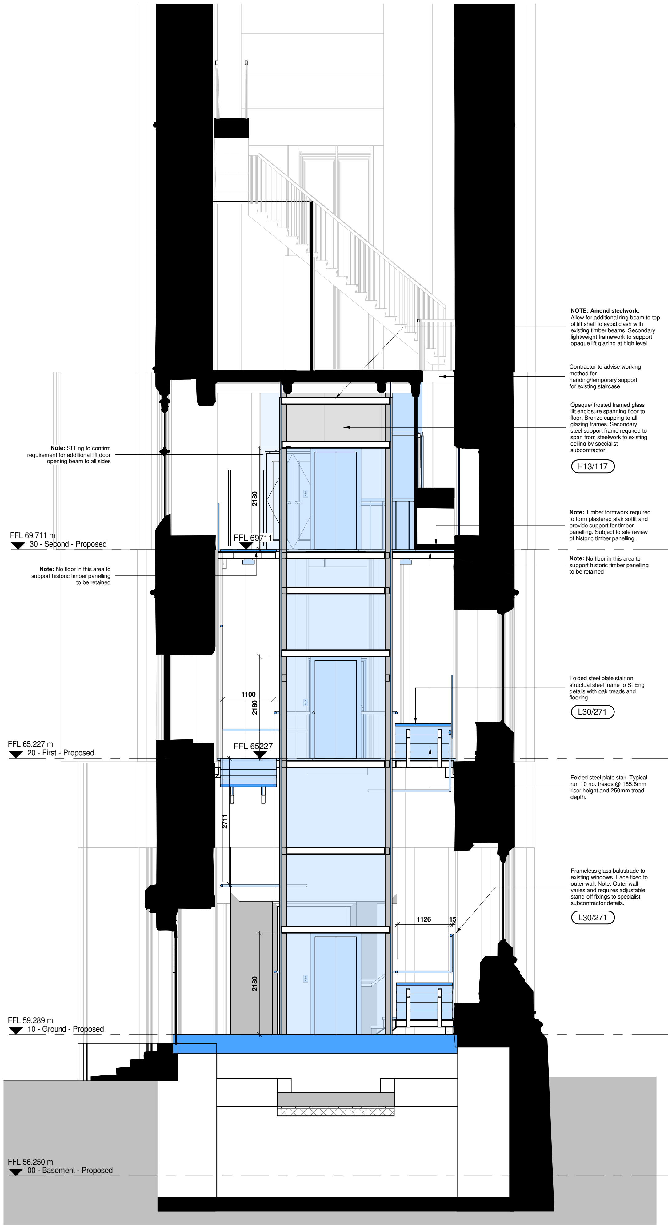
2D View 1 : 50
