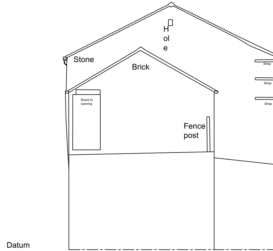
Elevation F
