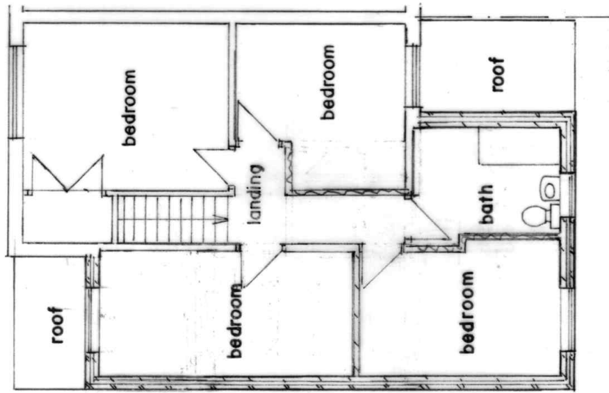
FIRST FLOOR PLAN (PROPOSED)
