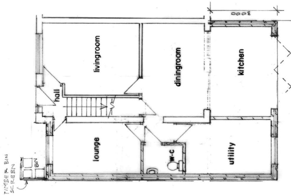
GROUND FLOOR PLAN (PROPOSED)
