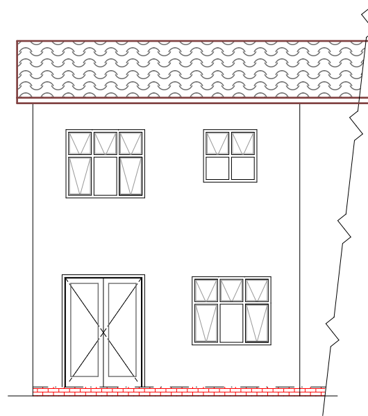
Rear Elevation 1:100
