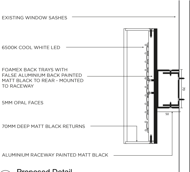
3 Proposed Detail Scale: 1:5
