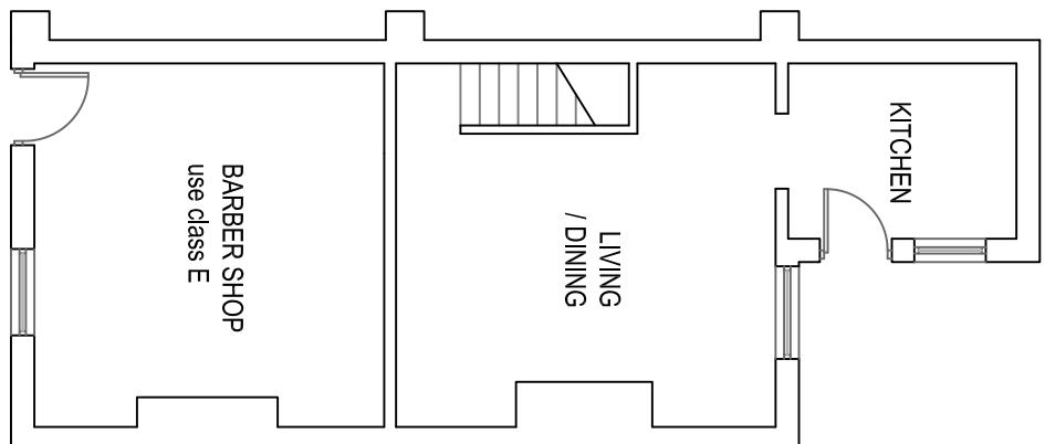
PROPOSED GF PLAN 1:100
