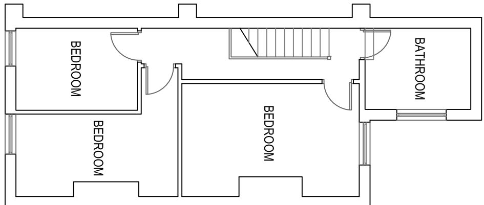
EXISTING FF PLAN 1:100
