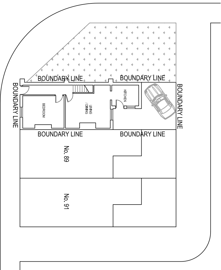
EXISTING SITE PLAN 1:200
