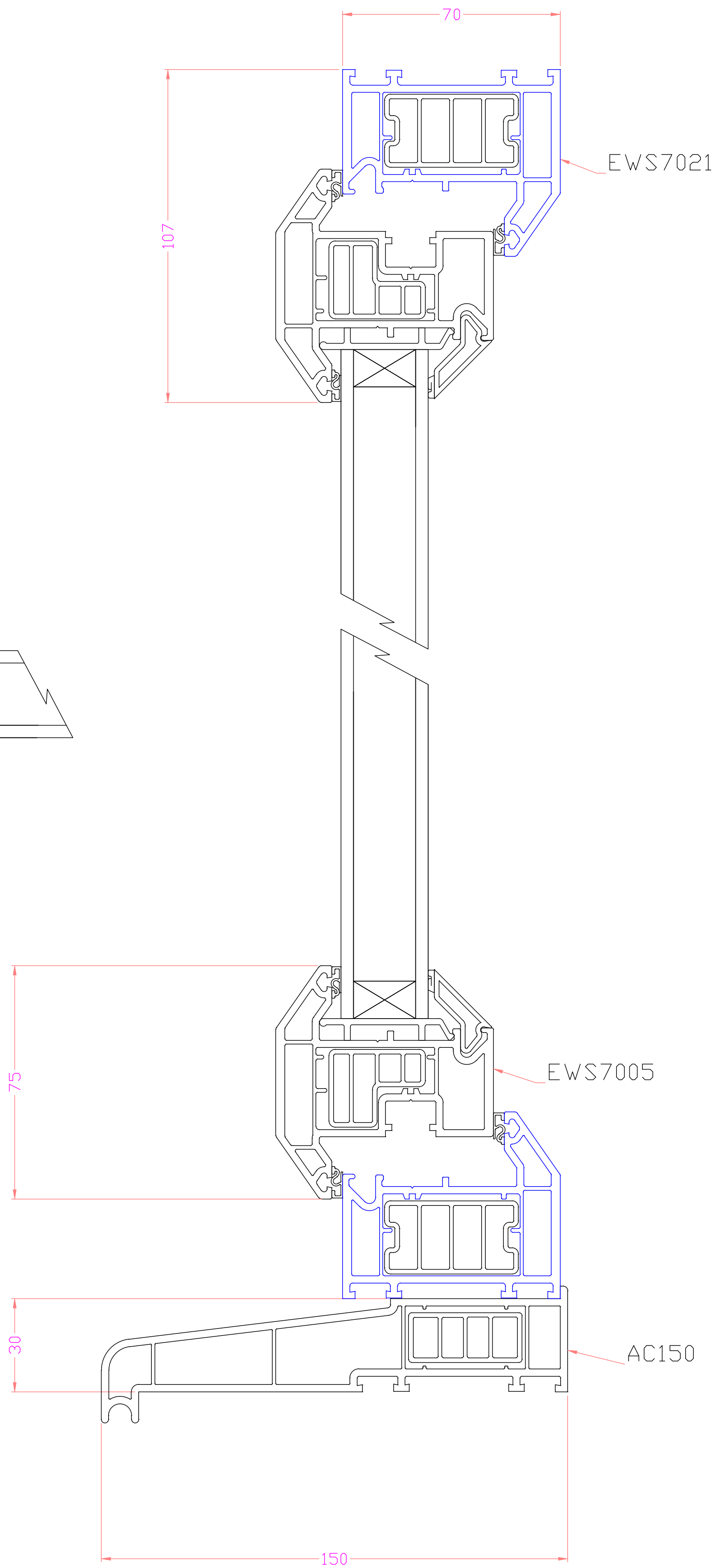
Section Y-Y
