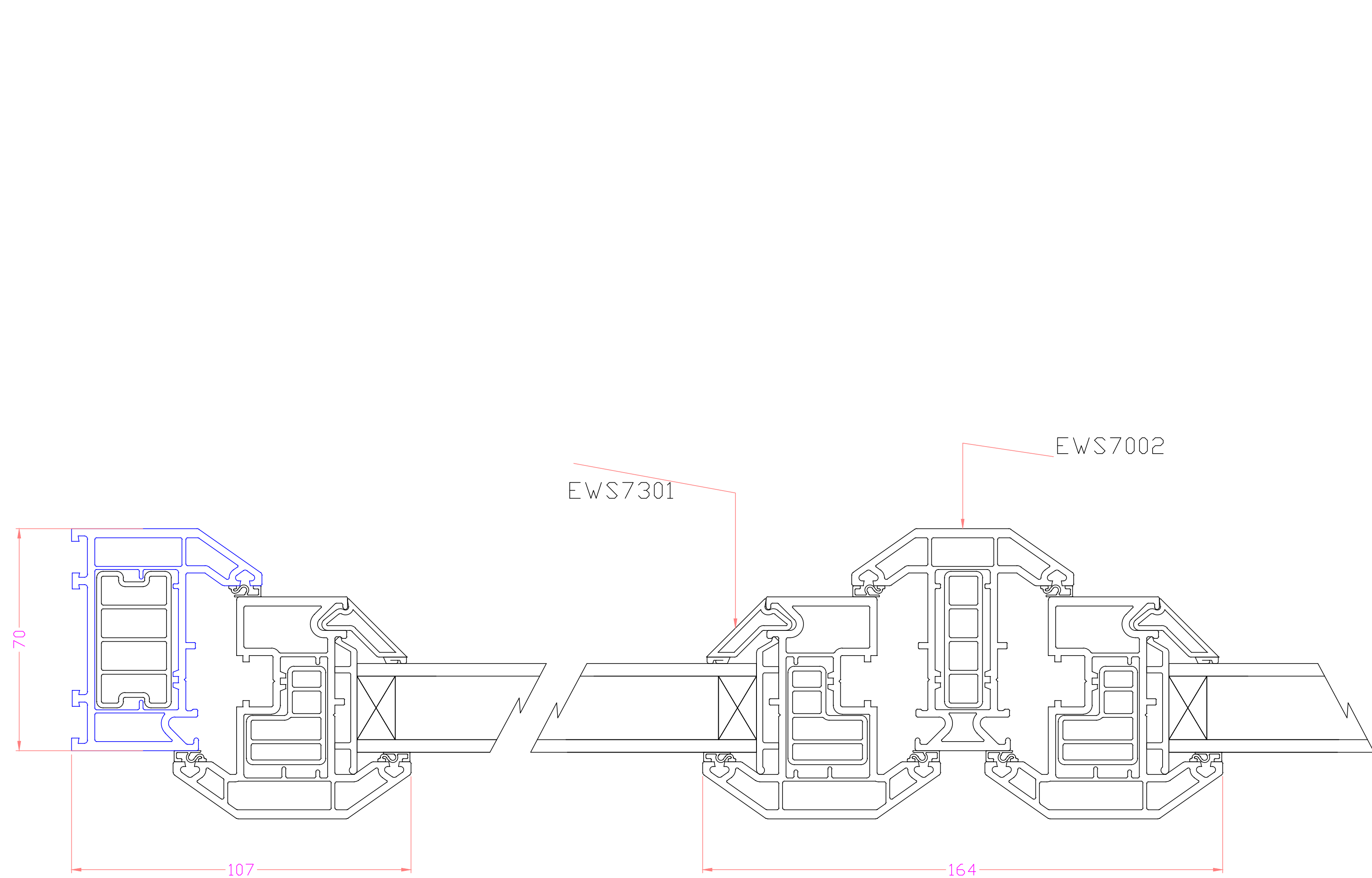
Section X-X
