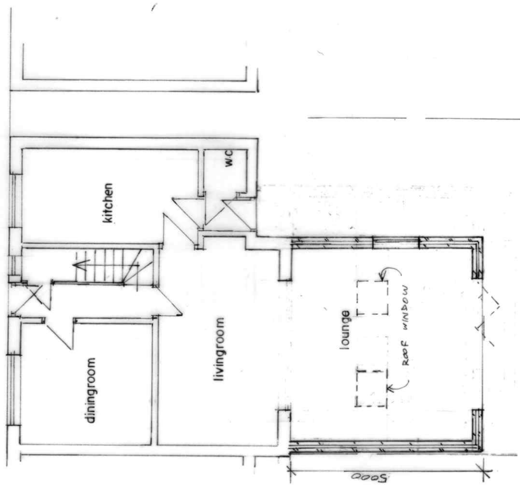
GROUND FLOOR PLAN (PROPOSED)
