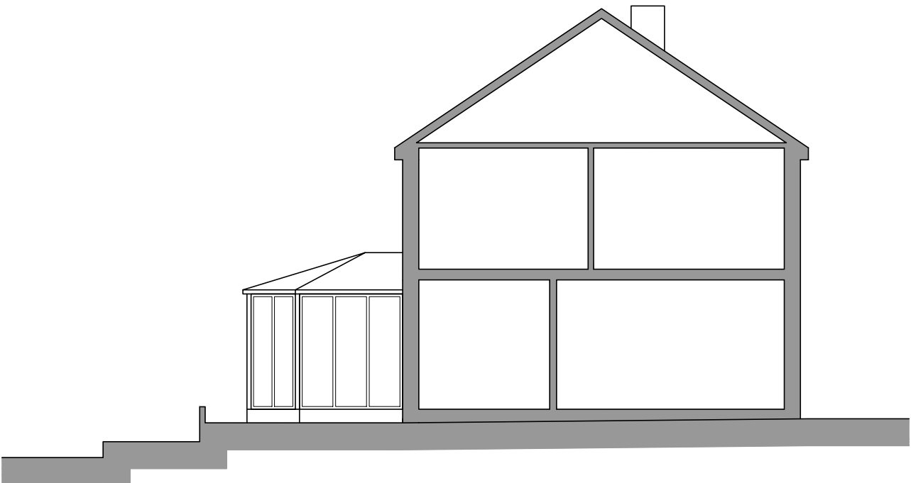
North Facing Side Elevational Section
