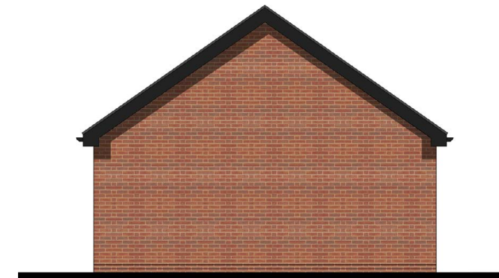
Side Elevation
