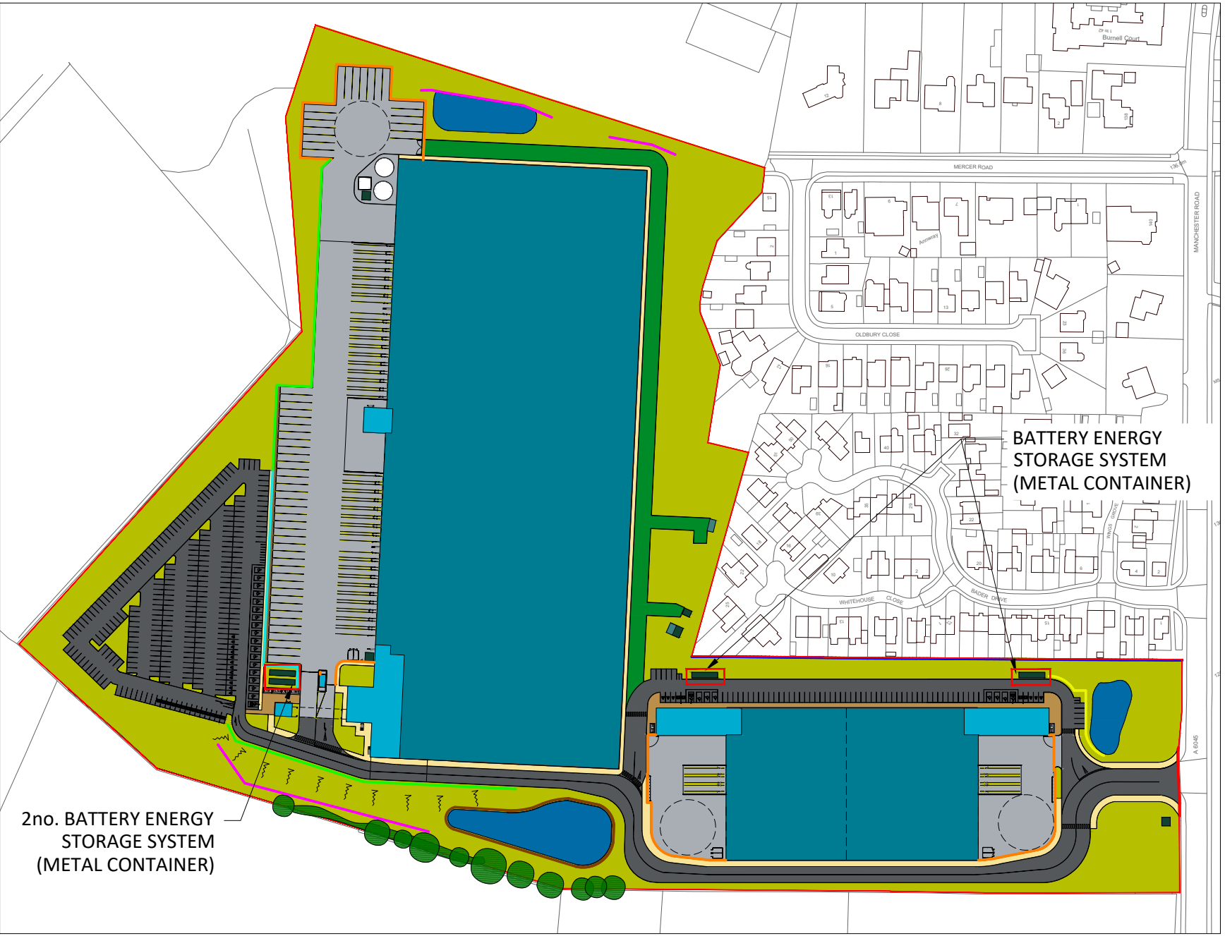
LOCATION PLAN 1:2500
