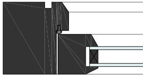
Jamb: Outward Opening Window
