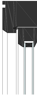
Head: Outward Opening Window
