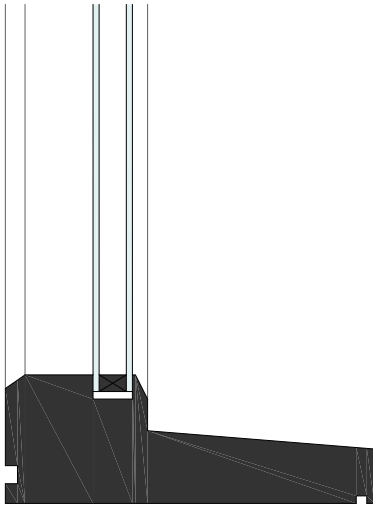
Sill: Fixed Window
