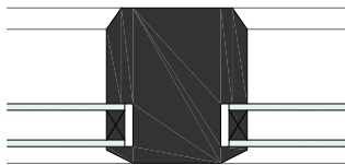
Vertical Mullion: Fixed Window
