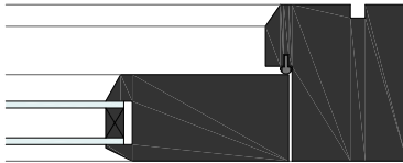
Jamb: Outward Opening Door
