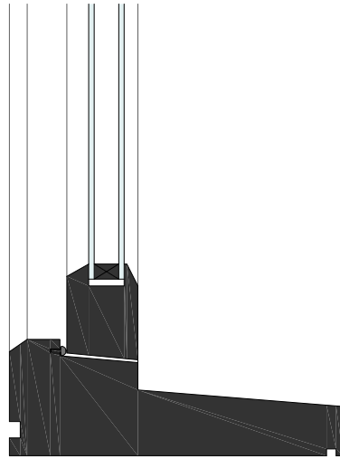
Sill: Outward Opening Window
