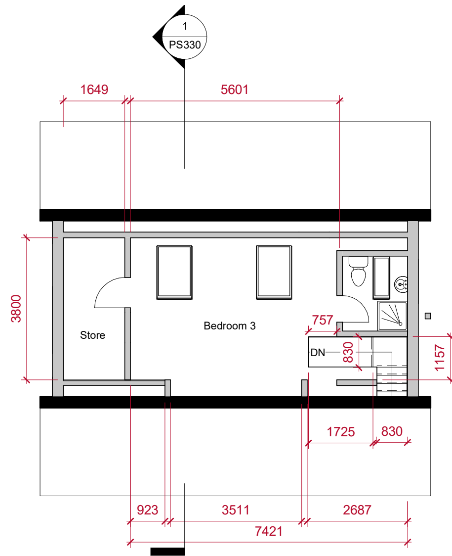
2 First Floor Plan 1 : 100
