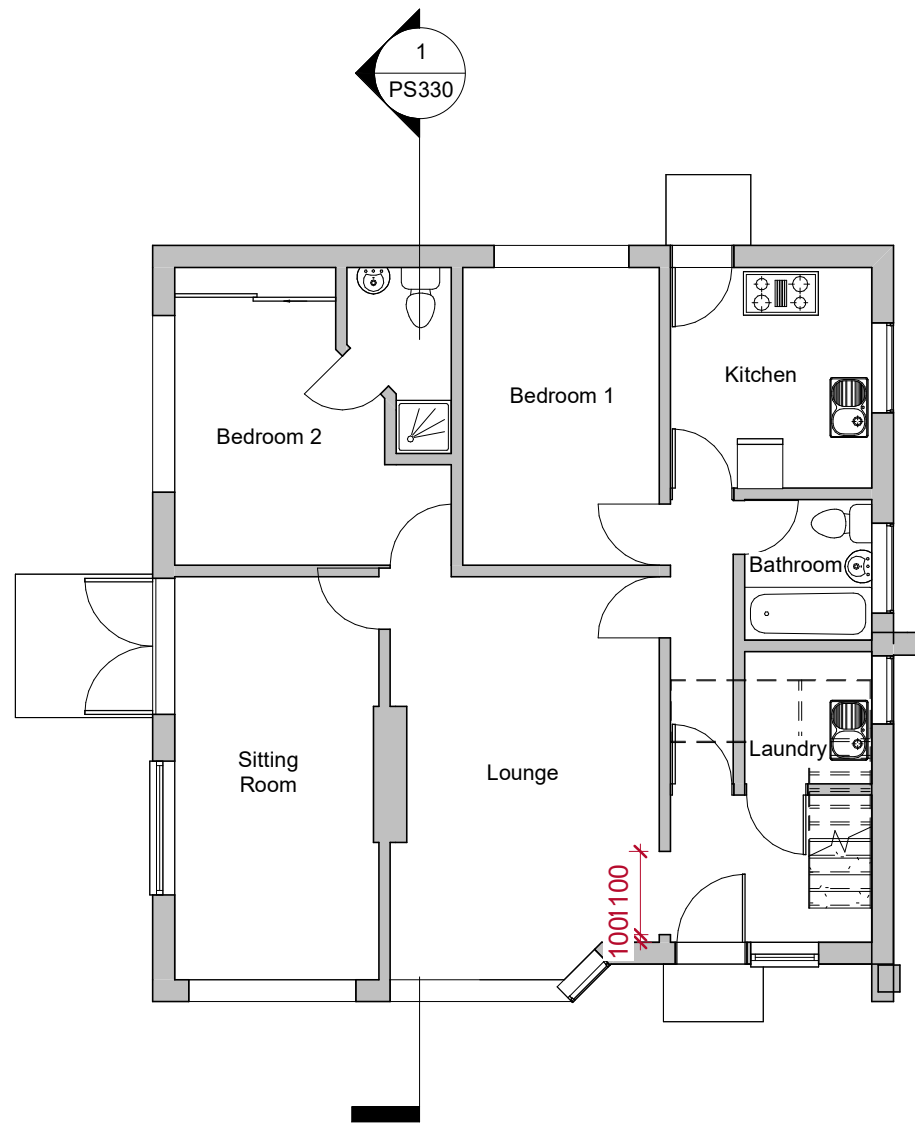
1 Ground Floor Plan 1 : 100
