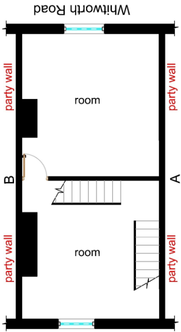
EXISTING FIRST FLOOR PLAN 1:50 @ A1
