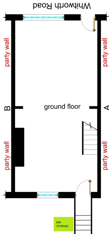
EXISTING GROUND FLOOR PLAN 1:50 @ A1
