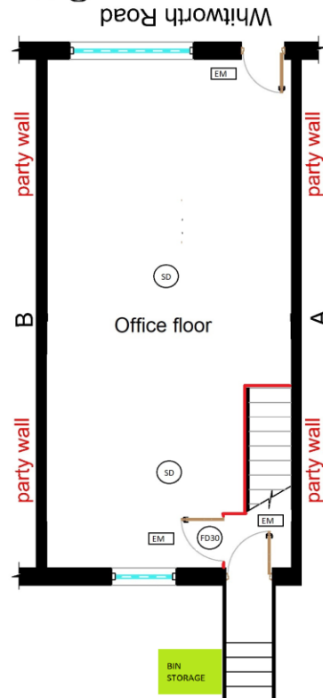
PROPOSED GROUND FLOOR PLAN 1:50 @ A1
