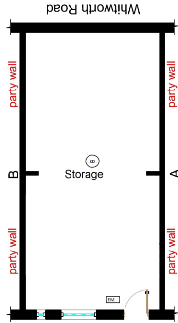
PROPOSED BASEMENT PLAN 1:50 @ A1
