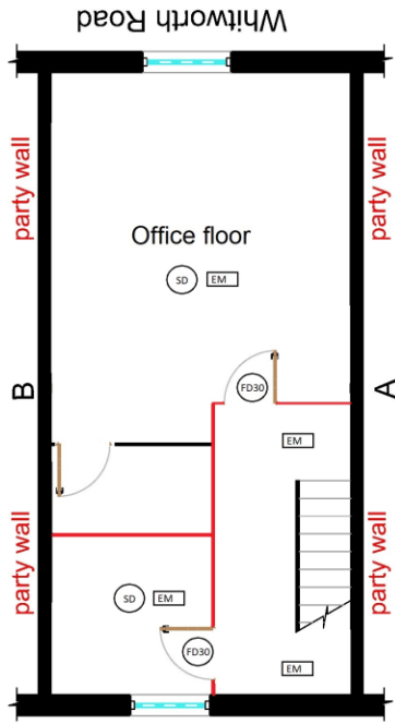
PROPOSED FIRST FLOOR PLAN 1:50 @ A1
