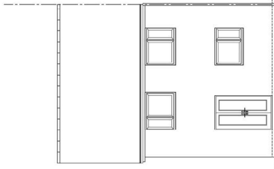
REAR ELEVATION END/SEMI DETACHED EMA33 (2B4F)
