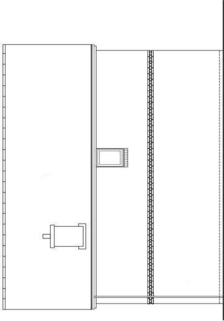
SIDE (RIGHT) ELEVATION DETACHED EMA35 (3B5P)
