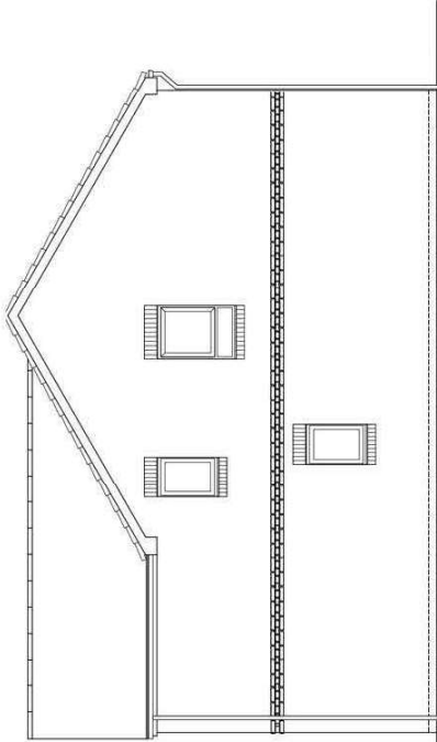
SIDE (RIGHT) ELEVATION DETACHED EMG43 (4B7F)
