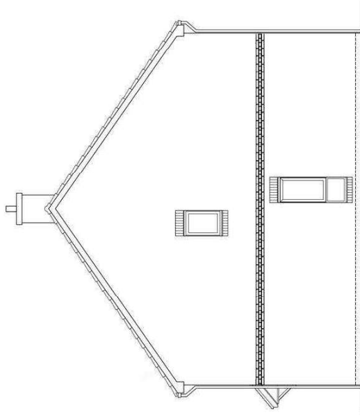
SIDE (RIGHT) ELEVATION DETACHED EMA43 (4B5P)
