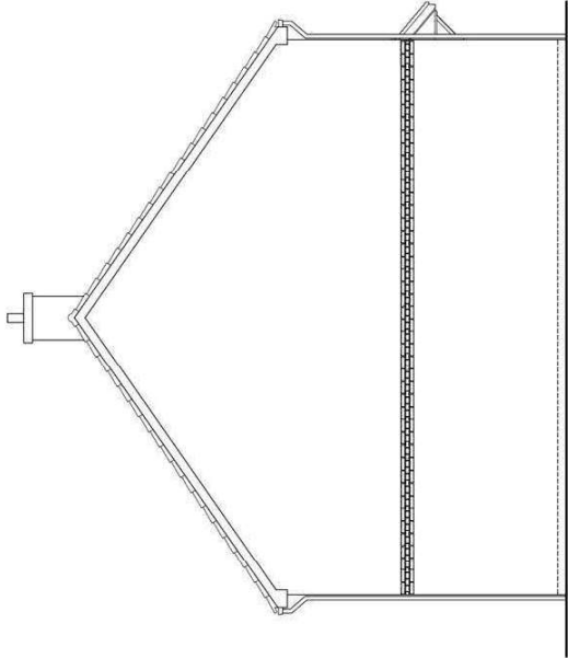
SIDE (LEFT) ELEVATION DETACHED EMA43 (4B5P)
