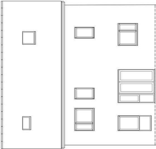
REAR ELEVATION DETACHED
