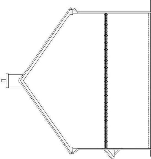
SIDE ELEVATION DETACHED EMA4G (4E7P)
