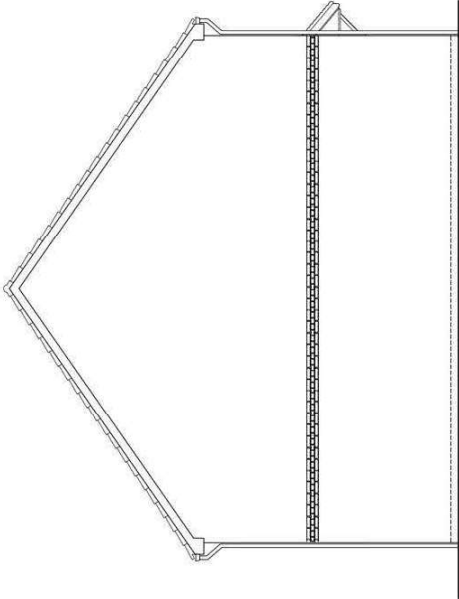
SIDE (LEFT) ELEVATION DETACHED EMA43 (4B5P)
