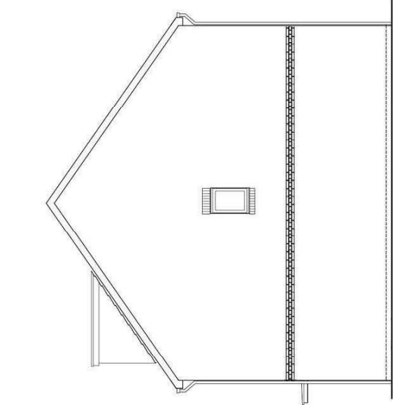
SIDE ELEVATION END/SEMI DETACHED EMB3 I (3B5P)
