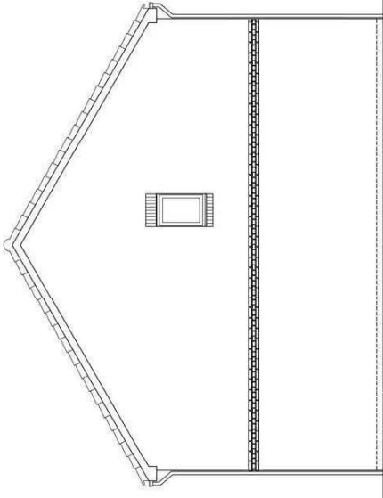
SIDE (RIGHT) ELEVATION END/SEMI DETACHED EMA35 (3B5P)
