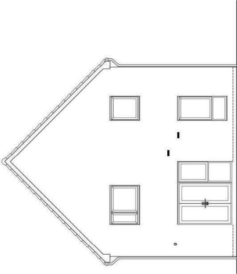
REAR ELEVATION DETACHED EMA43 (4B5P)
