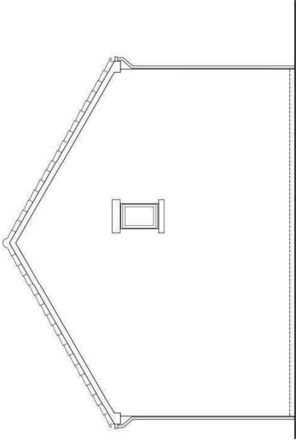
SIDE (RIGHT) ELEVATION END/SEMI DETACHED EMA35 (3B5P)
