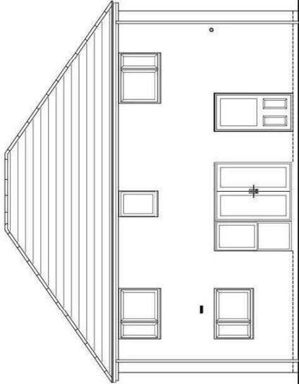
REAR ELEVATION DETACHED EMG43 (4B7F)
