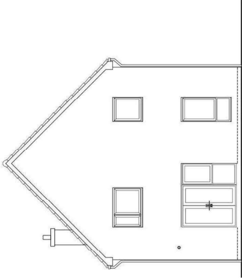
REAR ELEVATION DETACHED EMA43 (4BSF)
