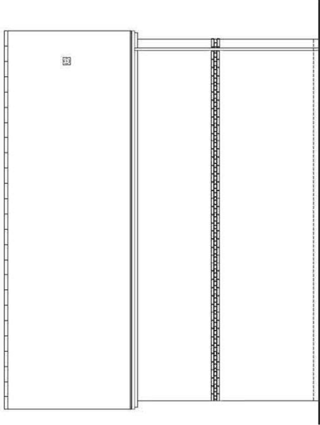
SIDE (LEFT) ELEVATION DETACHED EMA35 (3B5P)
