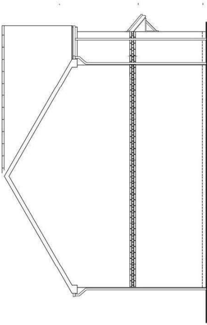
SIDE ELEVATION DETACHED EMG3 I (3B5F)
