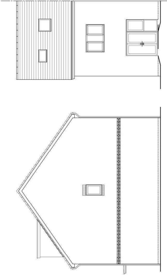
SIDE ELEVATION END/SEMI DETACHED EMB3 I (3B5P)
