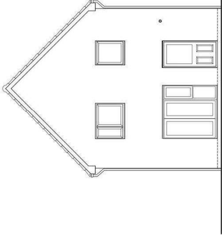
REAR ELEVATION DETACHED EMA35 (3B5P)
