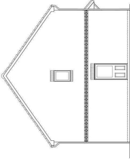
SIDE ELEVATION DETACHED EMA46 (4B7P)
