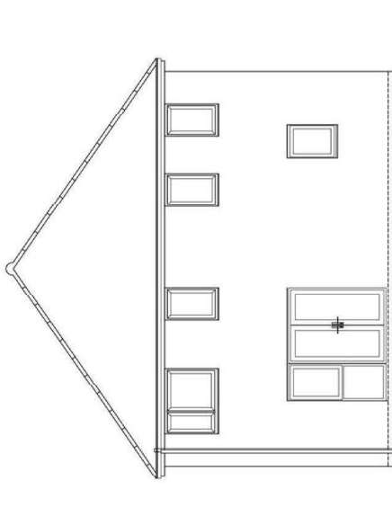
REAR ELEVATION DETACHED EMG31 (3BSF)
