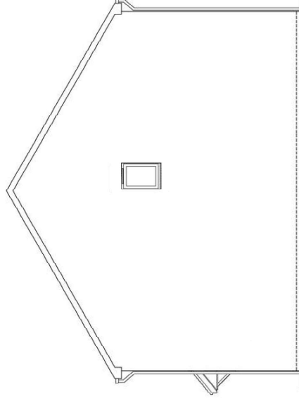
SIDE ELEVATION END/SEMI DETACHED EMA33 (2B4F)
