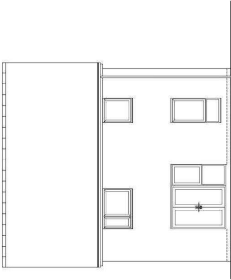
REAR ELEVATION DETACHED EMA43 (4B5P)
