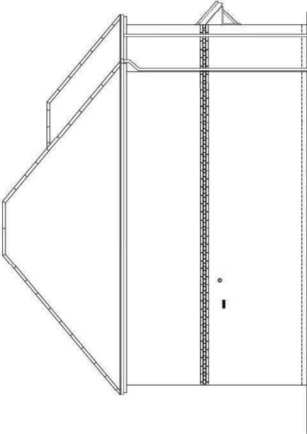
SIDE ELEVATION DETACHED
