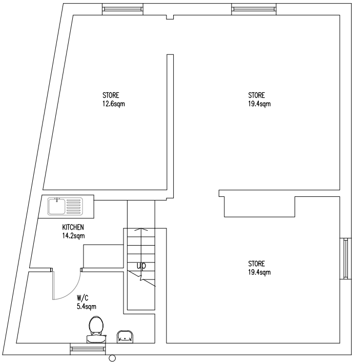
EXISTING FIRST FLOOR PLAN LAYOUT 1:100 © A3
