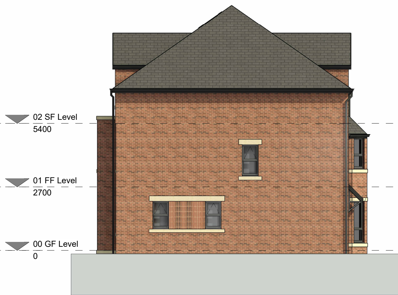
Left Elevation 1 : 100
