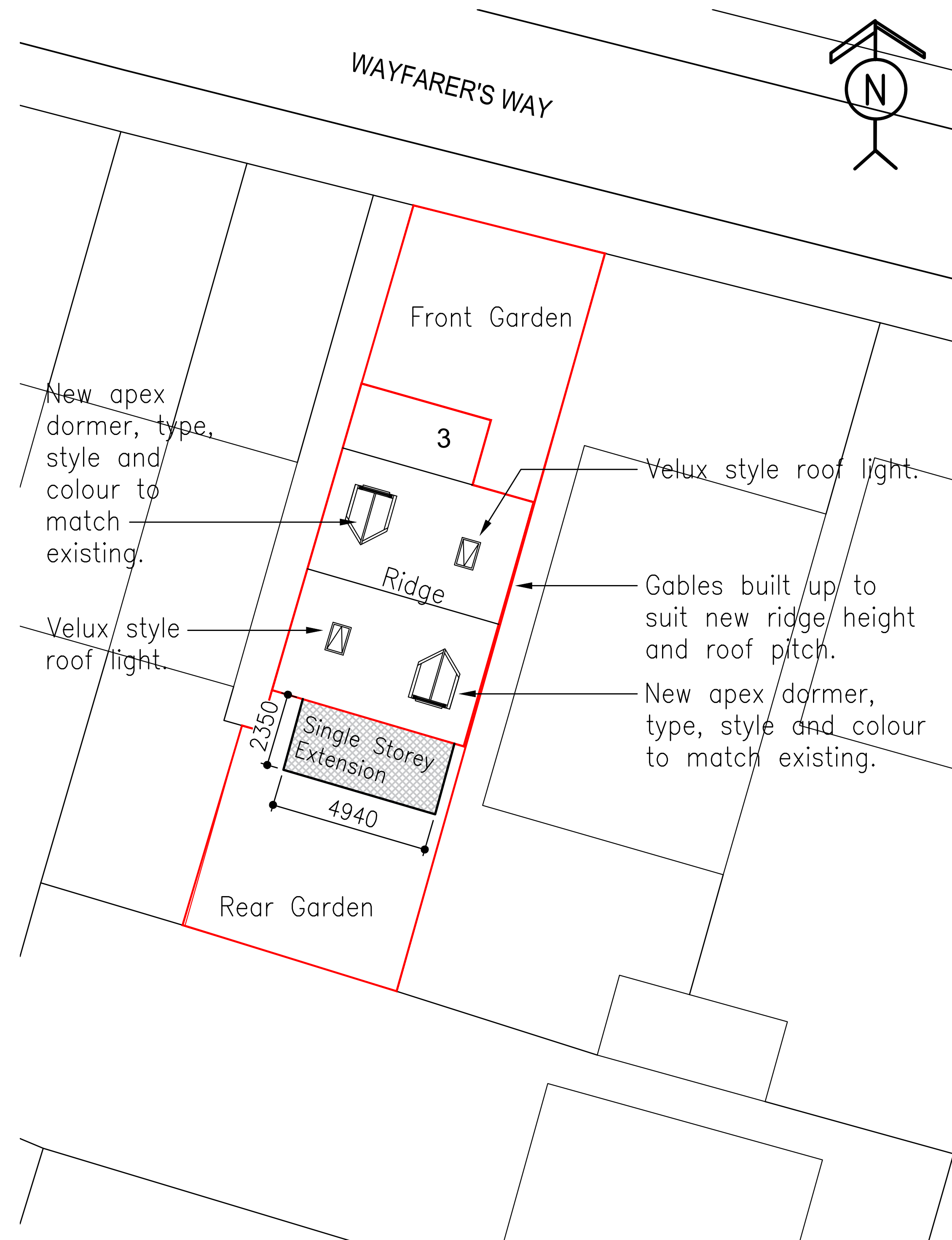
PROPOSED BLOCK PLAN
