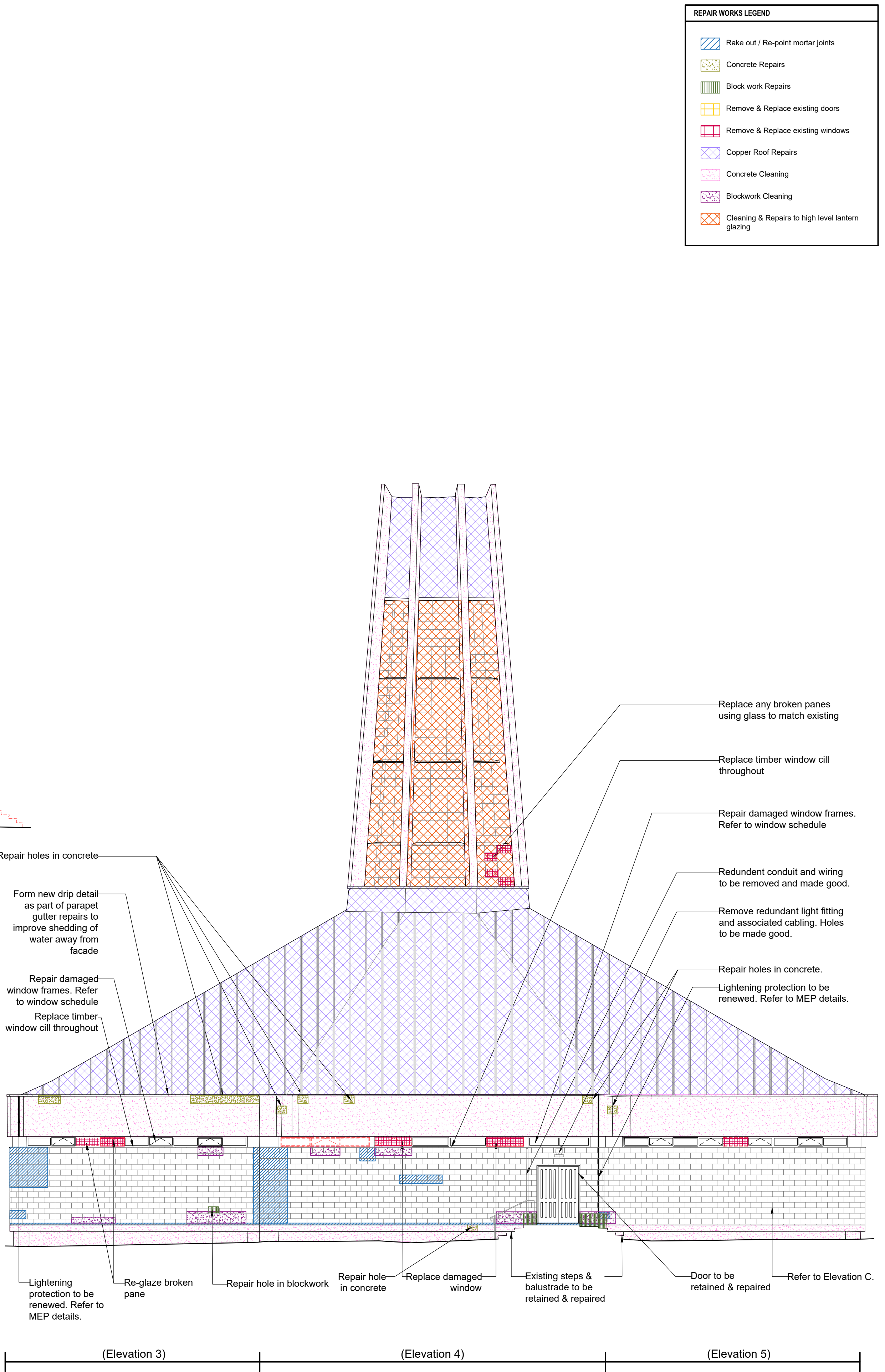
Elevation D
