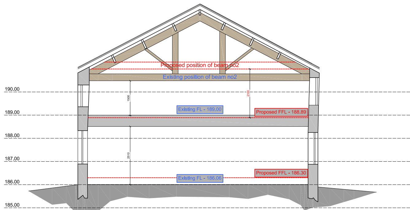
Existing & proposed position of beam 02
