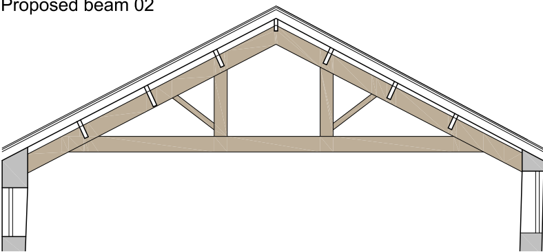
Proposed beam 02
