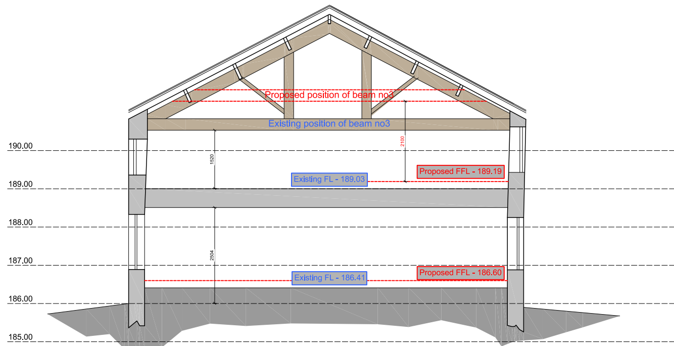
Existing & proposed position of beam 03
