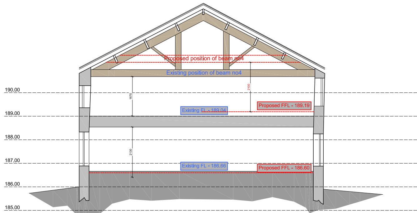
Existing & proposed position of beam 04
