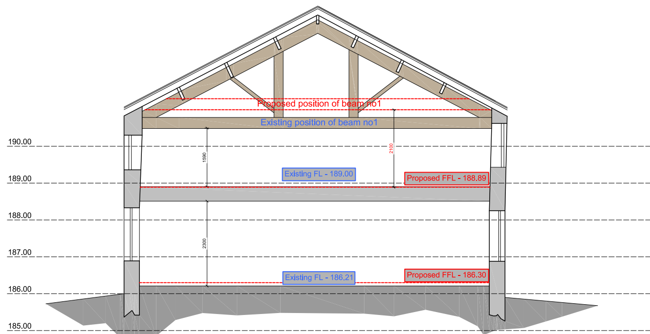
Existing & proposed position of beam 01
