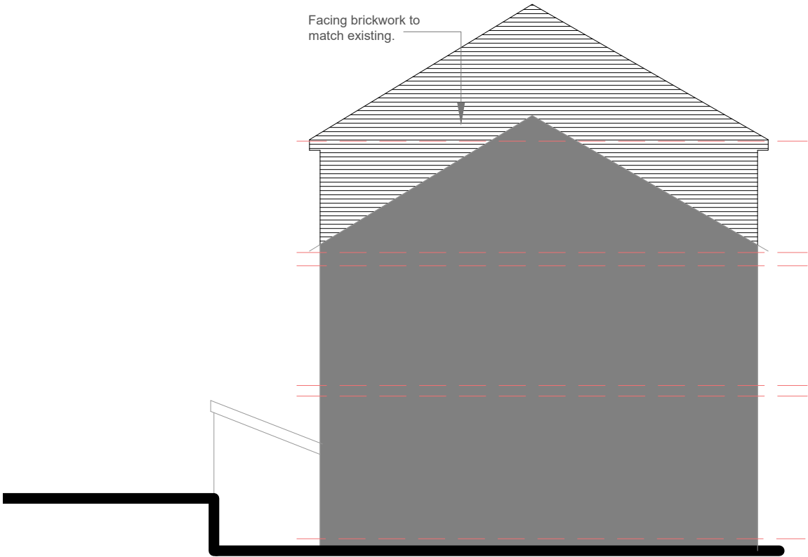
Side Elevation 1
