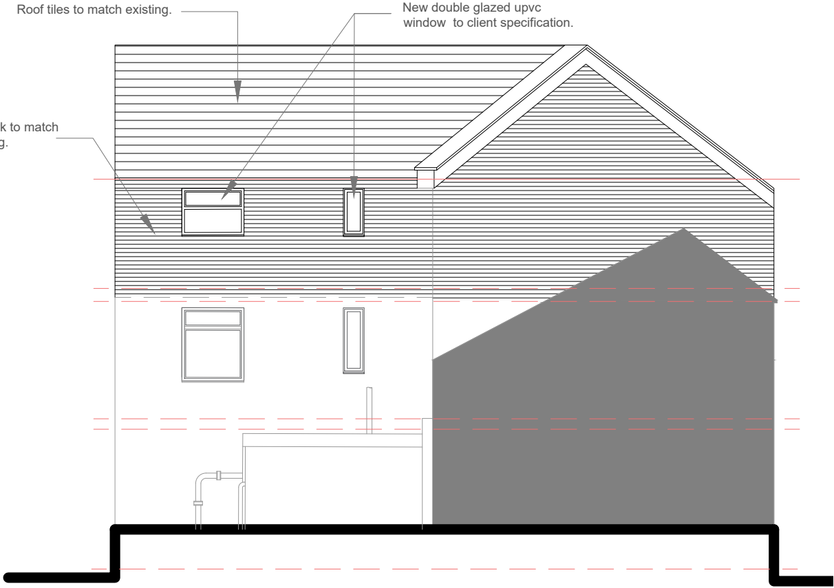
Rear Elevation
