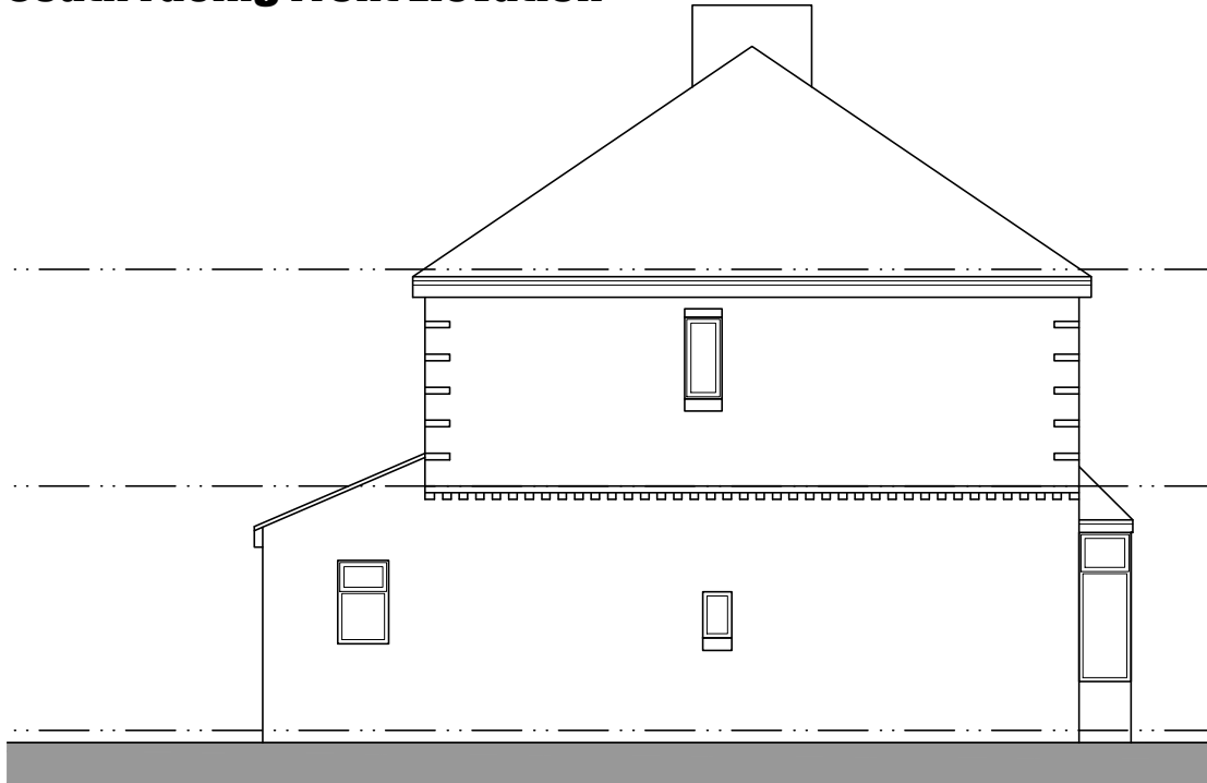
East Facing Side Elevation
